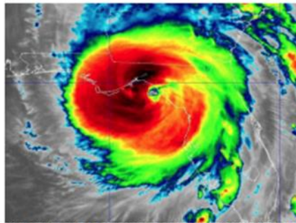
GOES-16 INFRARED IMAGE OF HELENE AT 0200 UTC 27 SEPTEMBER 2024 PRIOR TO LANDFALL IN FLORIDA. IMAGE COURTESY OF NOAA/NESDIS/STAR.
