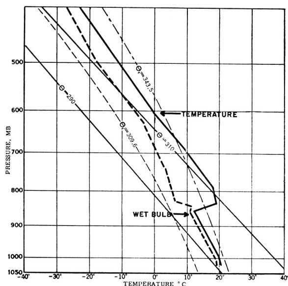
FIG. 4a. Upper-air sounding at Brownsville, Texas, 19 Feb. 1951, 0900 C.
