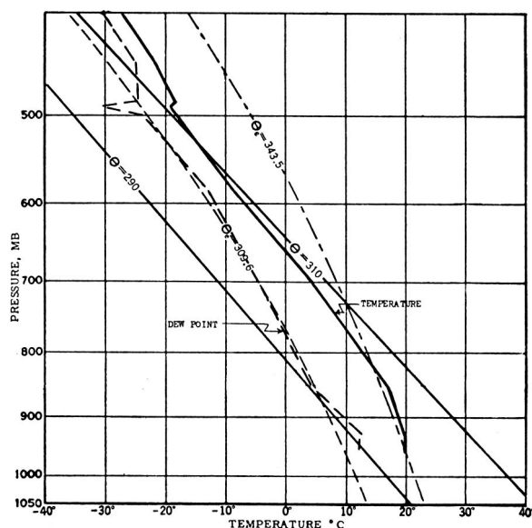
FIG. 10d. Upper-air sounding at Oklahoma City, Oklahoma, 2323 C, 11 April 1955.
