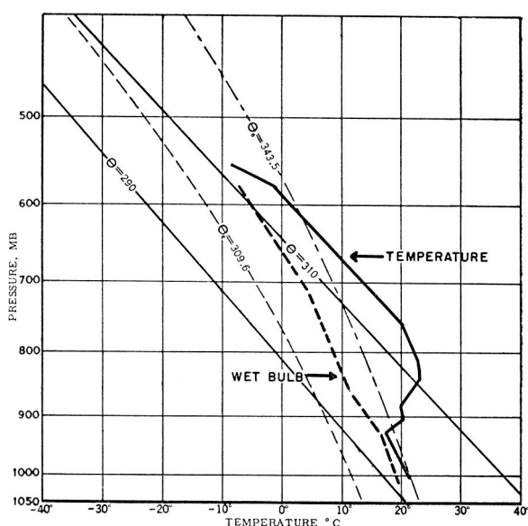
FIG. 4b. Upper-air sounding at Brownsville, Texas, 19 Feb. 1951, 2100 C.
