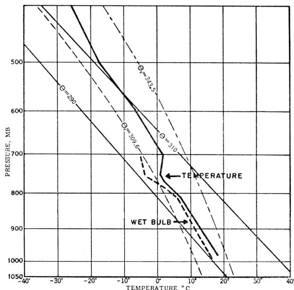
FIG. 2b. Upper-air soundings at Ft. Worth, Texas, 19 Feb. 1951, 2100 C (12 hr later than shown in 2a).
