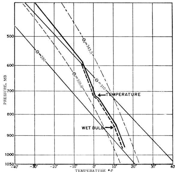
FIG. 2a. Upper-air soundings at Ft. Worth, Texas, 19 Feb. 1951, 0900 C.
