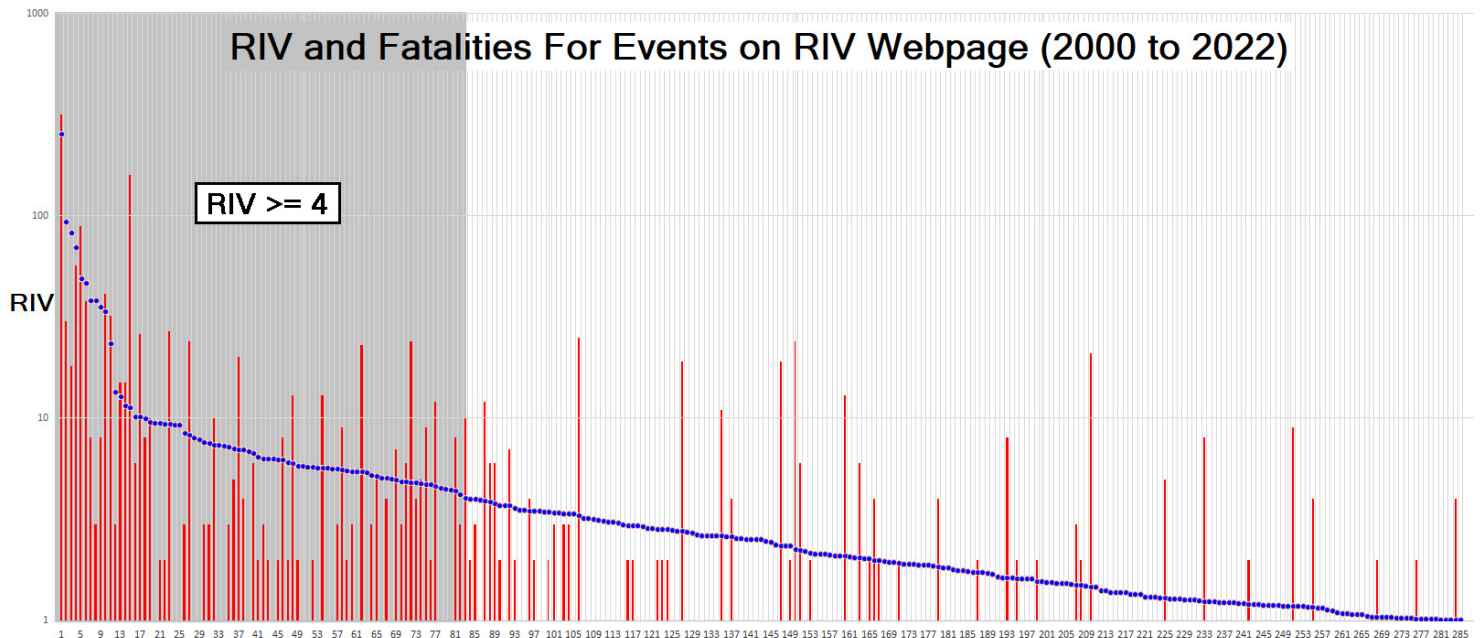
Figure 4. A graph showing RIV and fatalities for events in the RIV database from 2000 to 2022. RIV appears to be somewhat close to the fatality average for events with RIV \geq 4 . However, the variance in fatalities is large on the middle and right side of the chart, where event fatalities rarely end up near the average. For this reason, RIV is not considered a fatality estimate.
