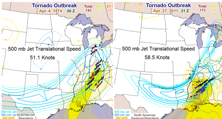
Figure 9. The 500 mb jet position at 00Z on April 4, 1974 (left), and the 500 mb jet position at 21Z on April 27, 2011 (right). In both cases, the 500 mb jet translation speed was above 50 knots. Tornado outbreaks associated with a 500 mb jet translation speed above 40 knots, have more potential to be high-end.
