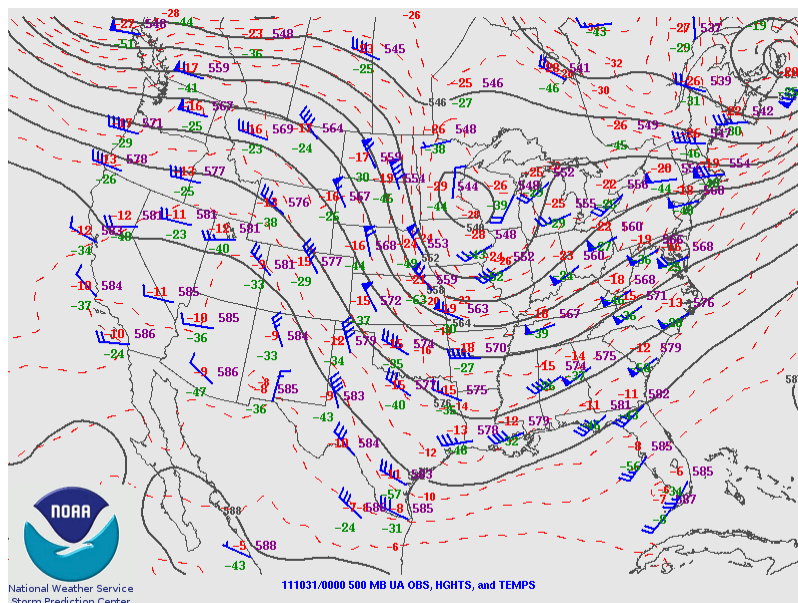
Figure 7. 500-mb observations and objectively-analyzed 500-mb heights (black), isotherms (dashed red), and wind bars (corresponding wind speeds in knots) at 0000 UTC 31 October 2011.
