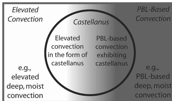
FIG. 11. Venn diagram of the relationship between elevated convection, PBL-based convection, and castellanus. The shading represents a gradation between elevated and PBL-based convection.
