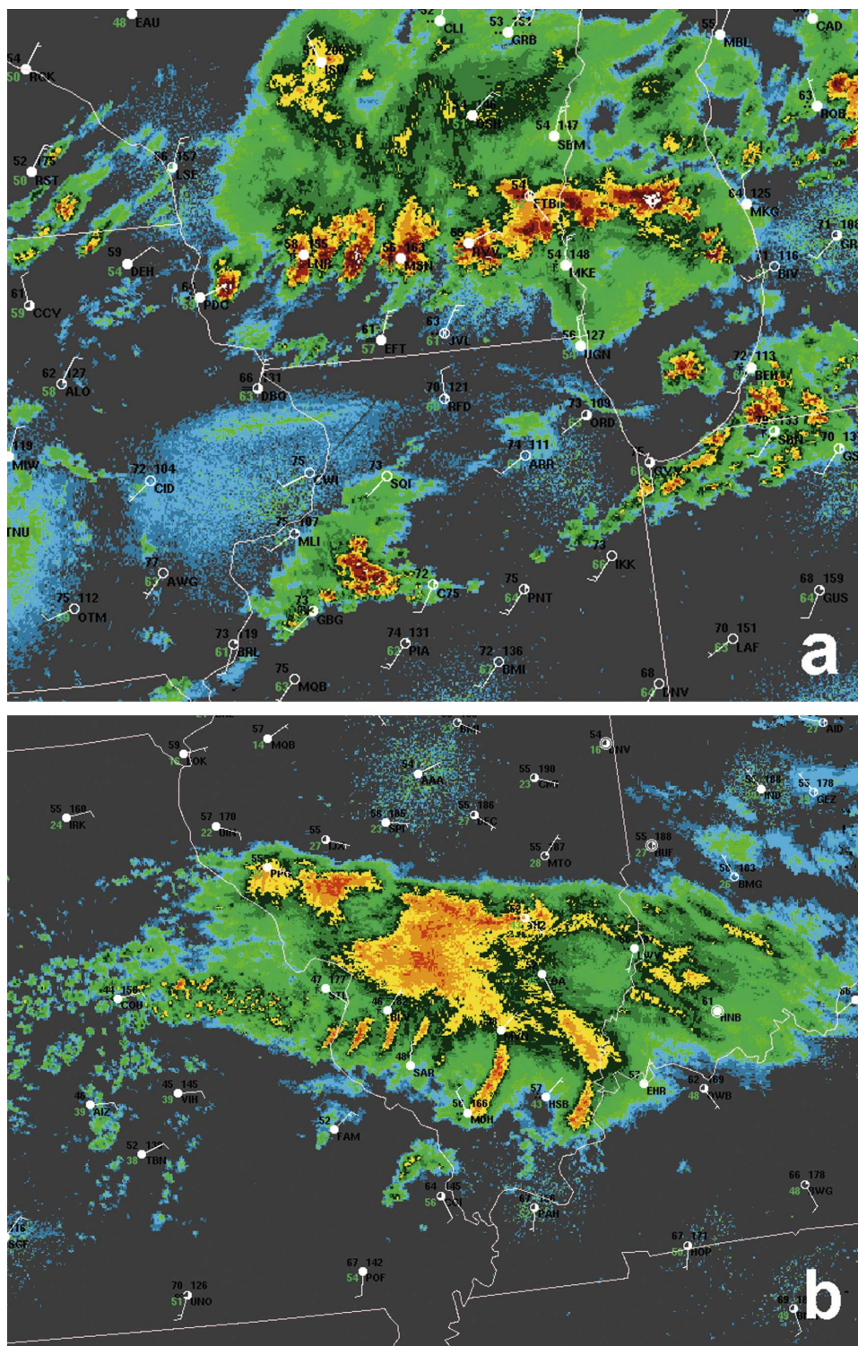
FIG. 9. (a) Composite reflectivity data showing a line of evenly spaced elevated thunderstorms, some supercells, over southern WI at 0600 CDT 4 Oct 2006. Conventional surface data locate west-east-oriented cold front along radar fineline over northern IL. Surface-based warm sector thunderstorms are present over northern IL and northwest IN. (b) Composite reflectivity data showing elevated showers and thunderstorms in short bands over southern IL at 1800 CDT 26 Mar 2008. Conventional surface data show west-east-oriented stationary front extending from southern MO into western KY.
