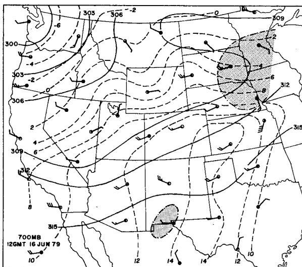
FIG. 5. 700 mb analysis valid at 1200 GMT, 16 June 1979. Solid lines are isohypes (dam), dashed lines are isotherms ( ^{\circ}\text{C} ), and stippling indicates 700 mb dewpoints greater than 0^{\circ}\text{C} .
