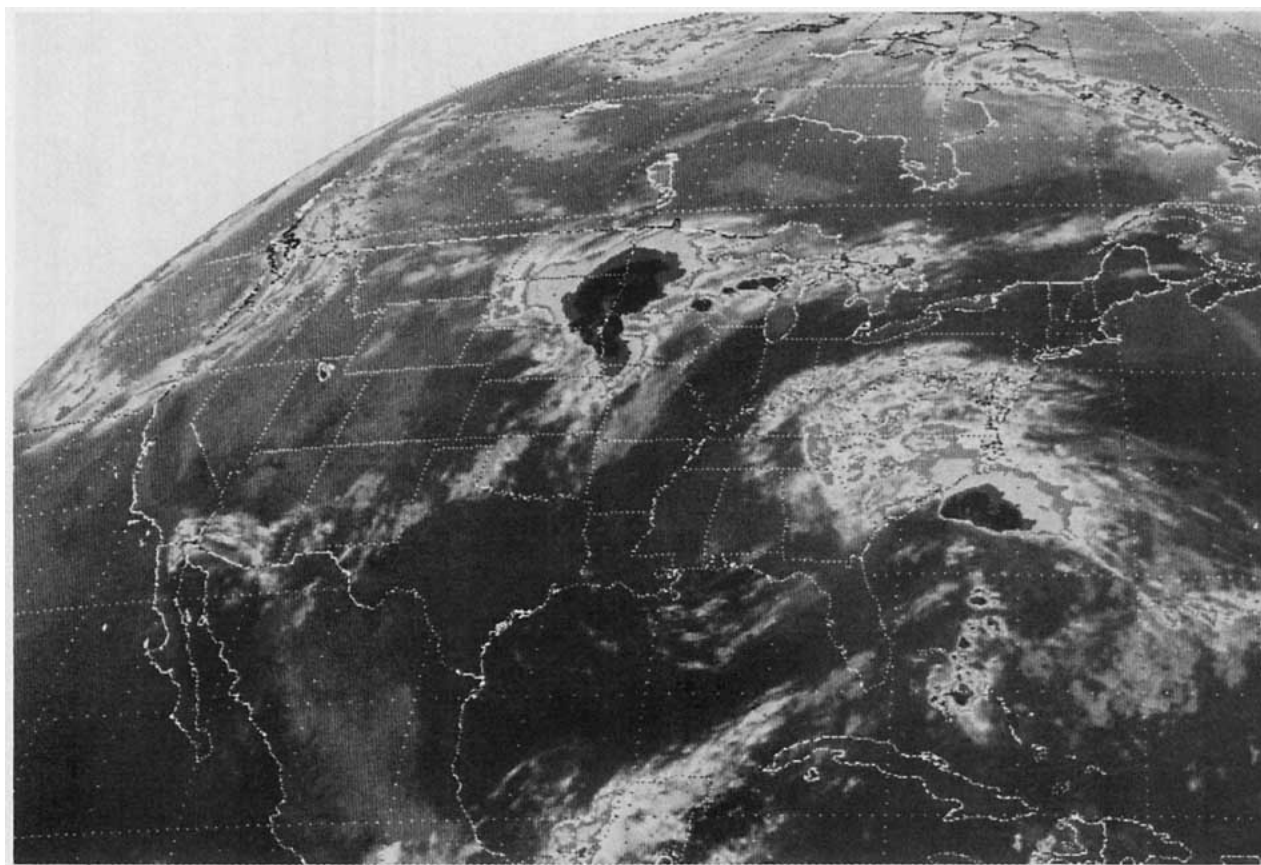
FIG. 3. Enhanced GOES infrared image at 1215 GMT, 16 June 1979.
