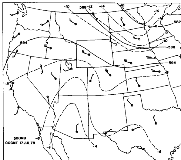
FIG. 19. As in Fig. 10, except on 17 July 1979.
