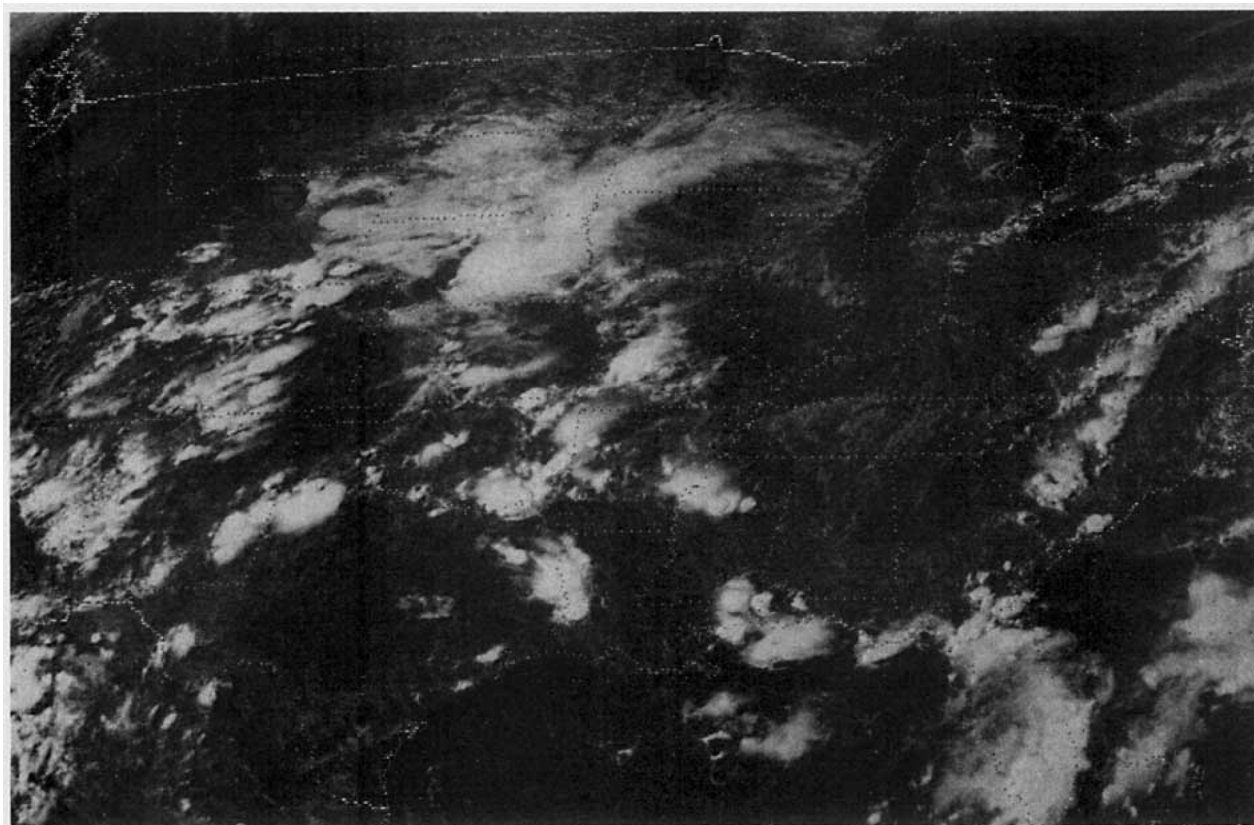
FIG. 16. As in Fig. 12, except at 2101 GMT.
