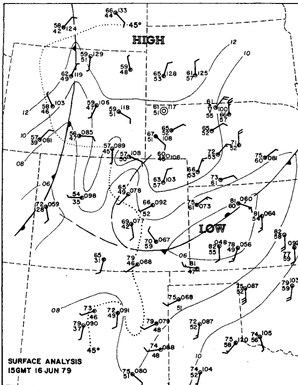
FIG. 4. Surface analysis valid at 1500 GMT, 16 June 1979. Symbols are conventional. Winds shown are peak gusts, when applicable. Dotted line denotes isodrosotherms ( ^{\circ}\text{F} ).
