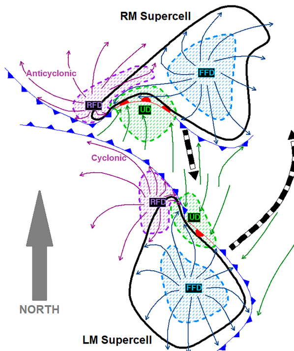
FIG. 3. Idealized LD79-type schematic of the RM supercell, and for the LM storm, similarly to Edwards and Hodanish (2006). Gust fronts labeled using conventional frontal symbology. Both supercells' shapes and relative positions are adapted to those herein at \approx 0110 UTC 29 May 2012. FFD stands for forward-flank downdraft, RFD for rear-flank downdraft, UD for updraft. Storm-relative surface flow is depicted by streamlines, with sign labeled in purple for areas behind the trailing part of each gust front. Inflow is green; outflow is blue (FFD) and purple (RFD). Thick black arrows represent supercell motion over the ensuing \approx 15 min.
