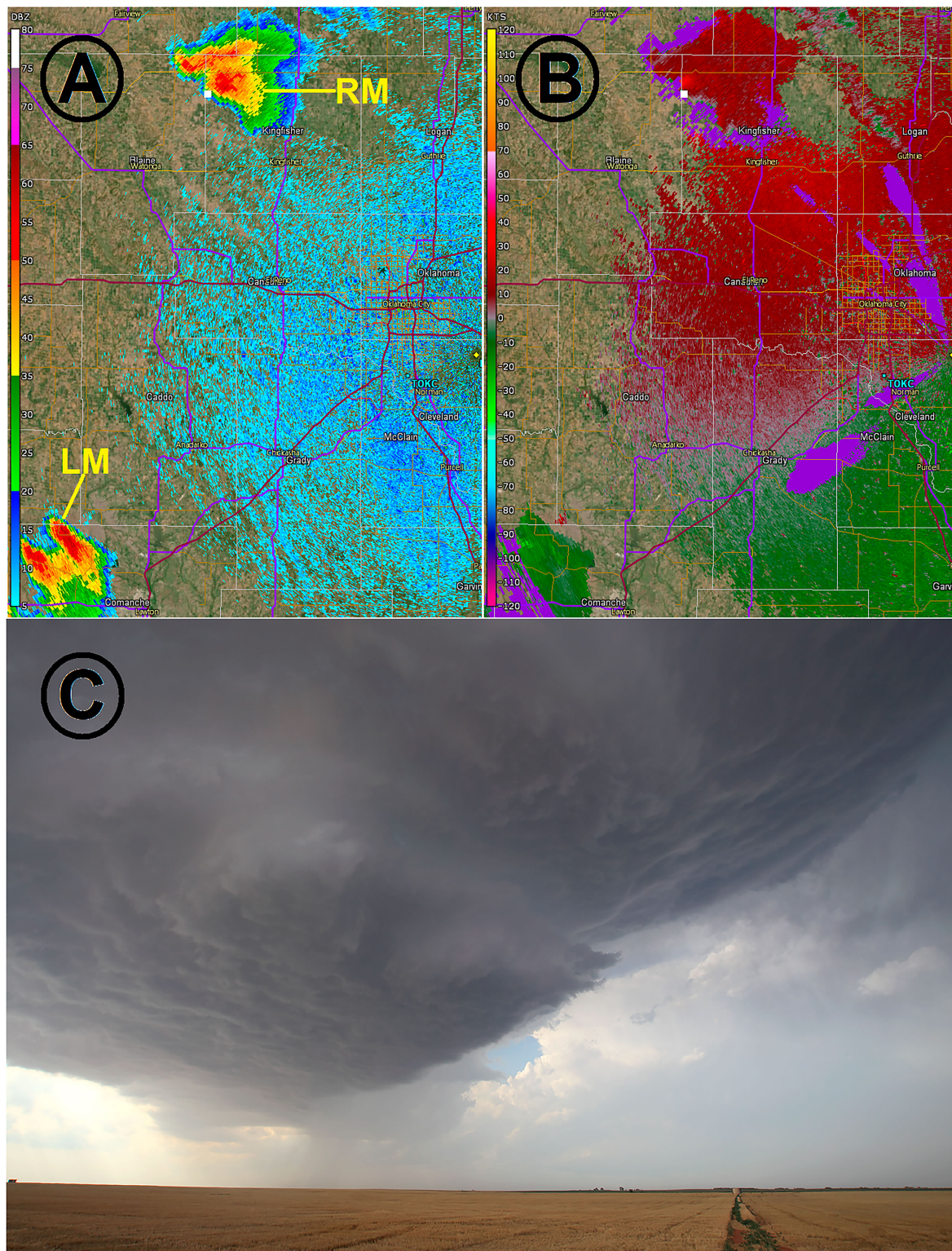
FIG. 4. All images at 2306 UTC 29 May 2012, with panels from the KTLX radar shown at 0.5^{\circ} beam elevation: (a) base reflectivity, (b) base velocity matching the spatial coverage of (a), (c) full-frame digital photograph looking north-northwest at 19-mm wide-angle focal length, showing a high-based wall cloud (which was rotating only weakly) from GPS location 36.058^{\circ} , -98.1974^{\circ} . (If pasting into mapping engine, use a hyphen for the negative value.) The yellow dot at the far right on the radar imagery denotes the radar location. The white square denotes the photo position next to the RM storm, with RM and LM storms labeled in (a). Radar display courtesy GRLevel2. (Photo by lead author R. Edwards.)
