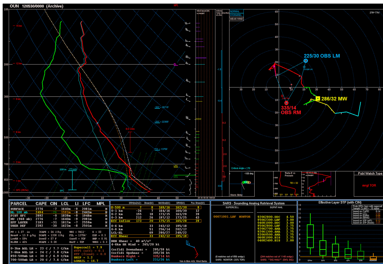
FIG. 1. Sounding for Norman, OK (OUN), 0000 UTC 30 May 2012, represented by (left) skew T -log p and (right) hodograph, with common SPC-NSHARP-derived parameters below, similar to the Python-based successor SHARPPy (Blumberg et al. 2017). Observed RM (thick red circle and label) and LM (thick blue circle and label) motions are added to the hodograph, with mean wind highlighted in yellow. Bunkers et al. (2000, 2014) RM and LM motions are represented by nearby, labeled, filled red and blue markers, respectively. Kinematic-related parameters are valid for the RM storm.
