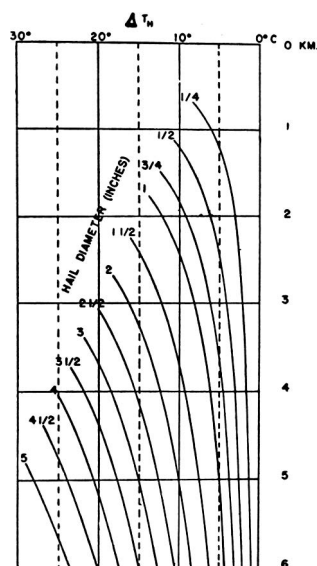
FIG. 3. Foster/Bates hail size diagram. Sizes shown are for -10^{\circ}\text{C} parcel temperature at 400 mb. Correct from FIGURE 4 for other levels. Diagram overlays WB Form 1147.
