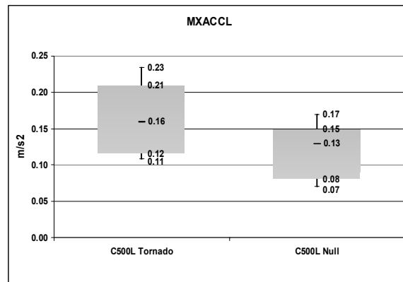
Fig. 10. Same as Fig. 2, except MXACCL ( \text{m/s}^2 ).
