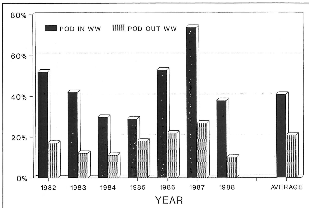
Fig. 8. POD of significant tornadoes in tornado warnings (dependent on the presence or absence of a tornado watch).
