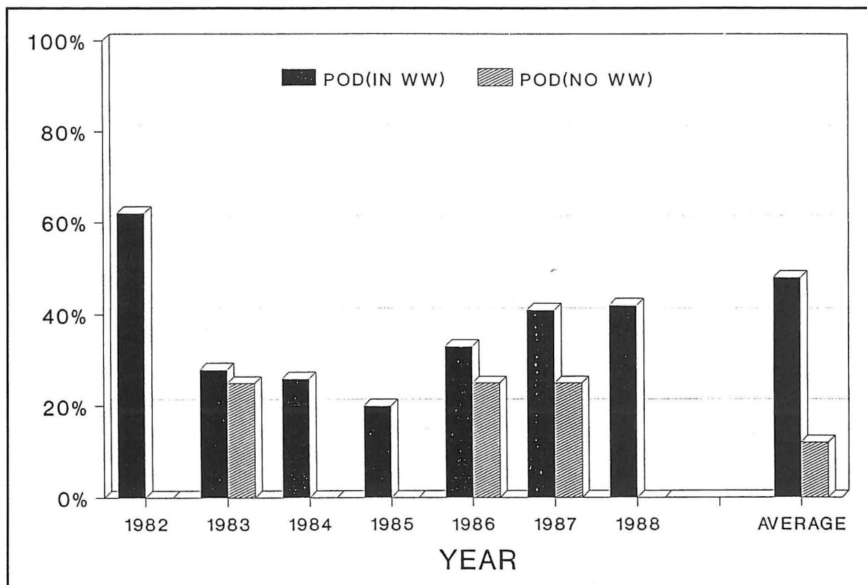
Fig. 7. POD of killer tornadoes in tornado warnings (dependent on the presence or absence of a tornado watch).
