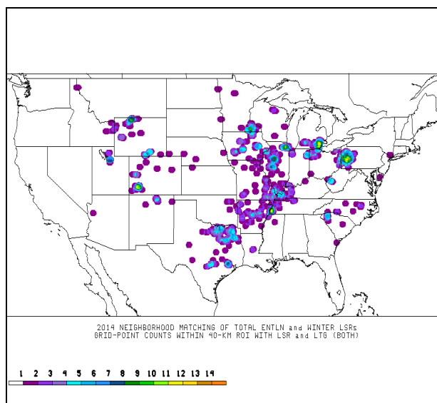
Figure 13: Same as in Fig. 12 except for neighborhood matching of total (CG+IC) ENTNLN and winter LSRs.
