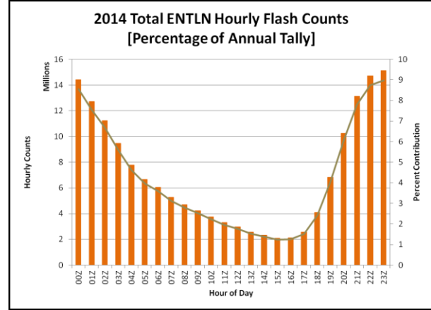
Figure 2: 2014 Total ENTNLN hourly flash counts (in millions) and percentages of annual tally.
