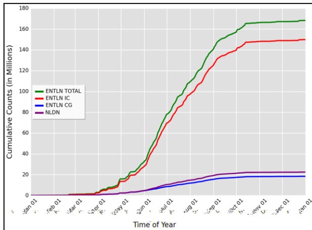
Figure 1: Running annual tally of hourly lightning flashes in 2014 from QC-CG NLDN. For comparison, total lightning counts from ENTNLN as well as the corresponding CG and IC flash components are provided.
