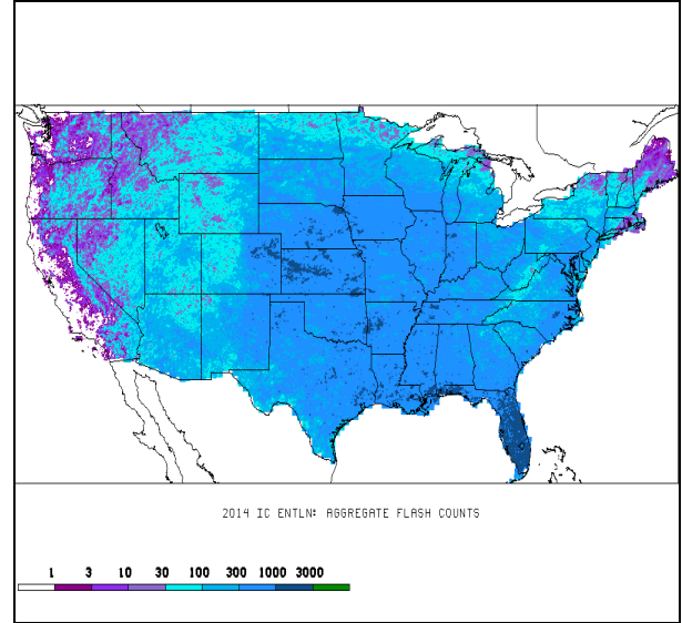
Figure 8: 2014 IC ENTNLN aggregate flash counts for the high-resolution grid covering the contiguous United States.
