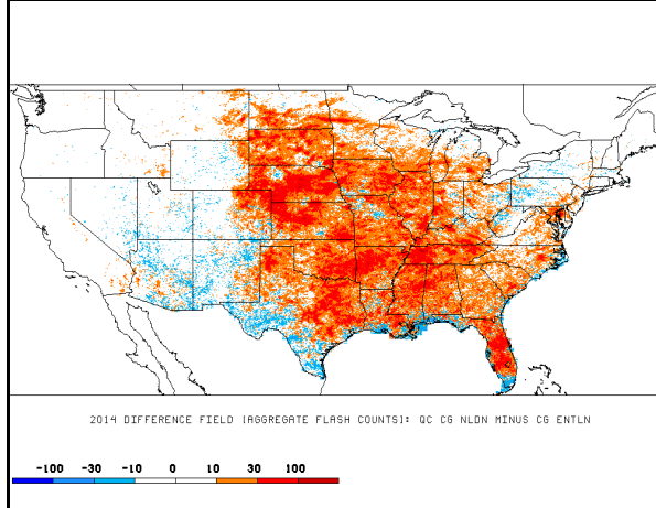
Figure 7: 2014 difference field of aggregate flash counts (QC-CG NLDN – CG ENTNLN).
