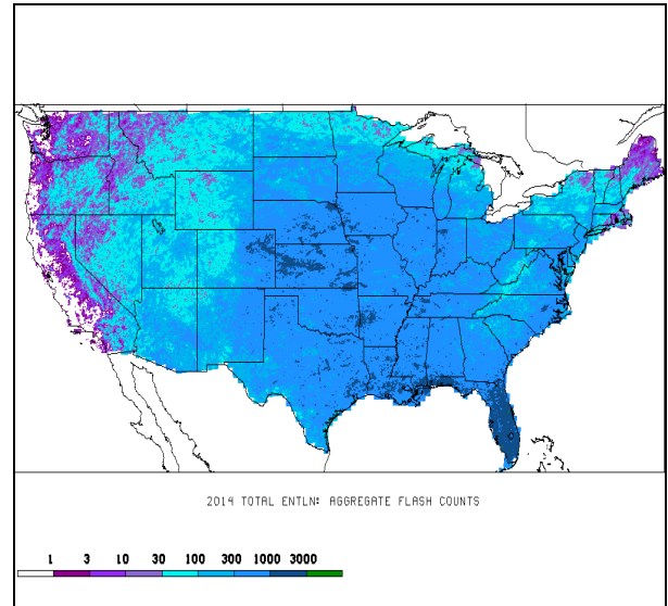
Figure 9: Same as in Fig. 8 except for 2014 Total (CG+IC) ENTNLN aggregate flash counts.
