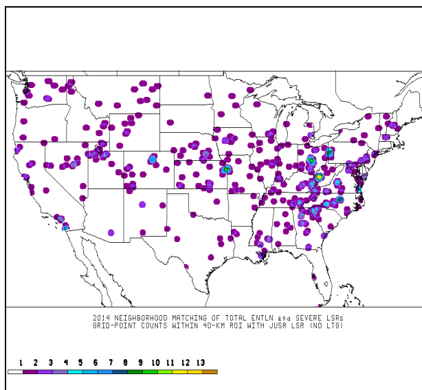
Figure 11: Same as in Fig. 10 except for neighborhood matching of total (CG+IC) ENTNLN and severe LSRs.
