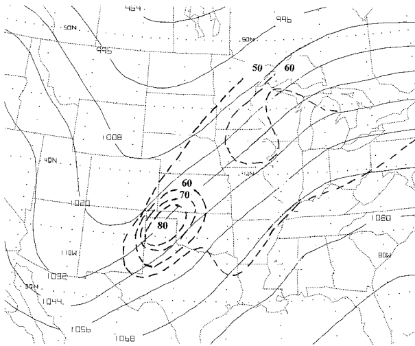
FIG. 3. The 250-hPa geopotential height and isotach analysis valid 1200 UTC 1 Mar 1997. Solid lines represent height values in dm with dashed lines indicating isotachs in \text{m s}^{-1} .
