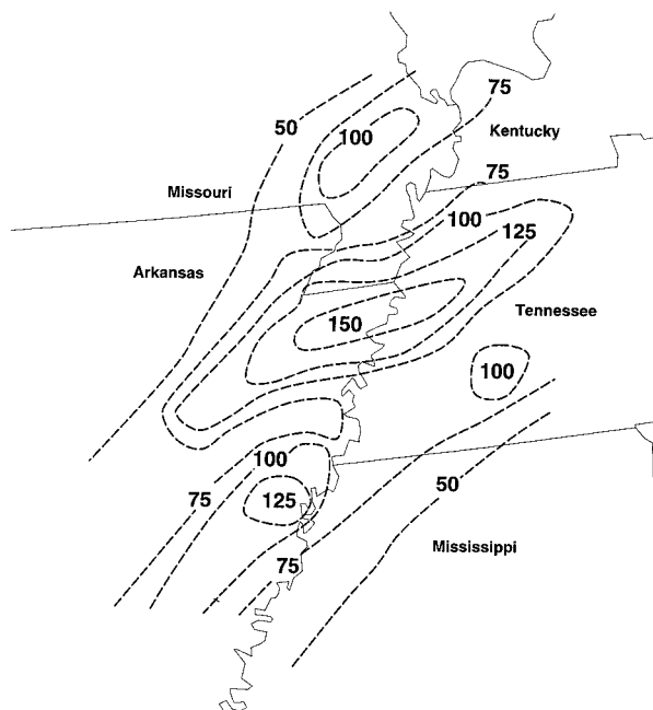
FIG. 2. The 24-h total rainfall (mm) for eastern Arkansas, western Tennessee, and adjacent areas ending at 1200 UTC 2 Mar 1997. Measurements based on NWS cooperative rain gauges.
