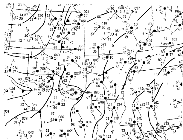
FIG. 7. Subjective surface analysis at 1200 UTC 1 Mar 1997. Temperature and dewpoint are in ^{\circ}\text{F} with pressure in mb (using standard abbreviations). The 3-h pressure tendencies (in tenths of mb) also included.
