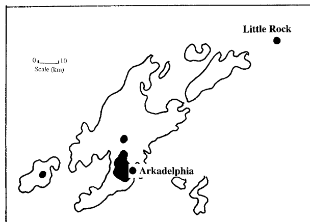
FIG. 21. KLZK base reflectivity image at 2042 UTC for the Arkadelphia–Little Rock area during the time of the Arkadelphia tornado. Other details the same as in Fig. 20.
