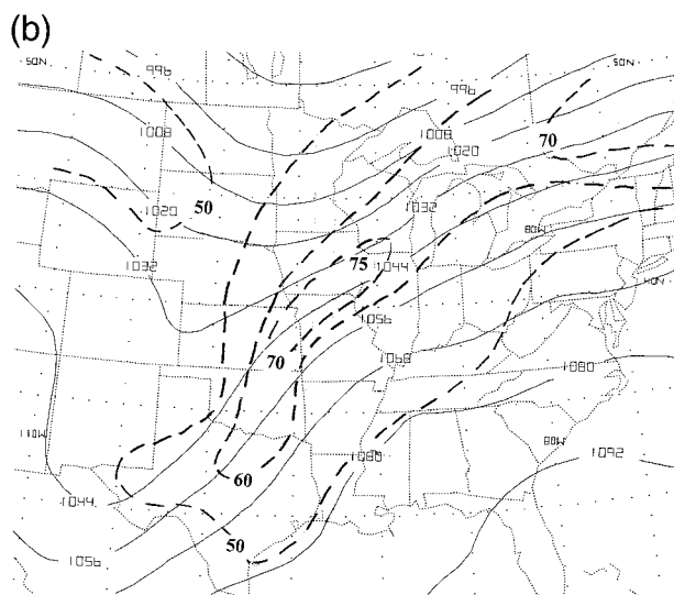
FIG. 8. The 250-hPa geopotential height and isotach analyses for (a) 1800 UTC 1 Mar 1997 based on 6-h Eta Model forecast and (b) 0000 UTC 2 Mar 1997 based on observational data. Solid line in (a) indicates orientation of cross section in Fig. 16. Other details the same as in Fig. 3.
