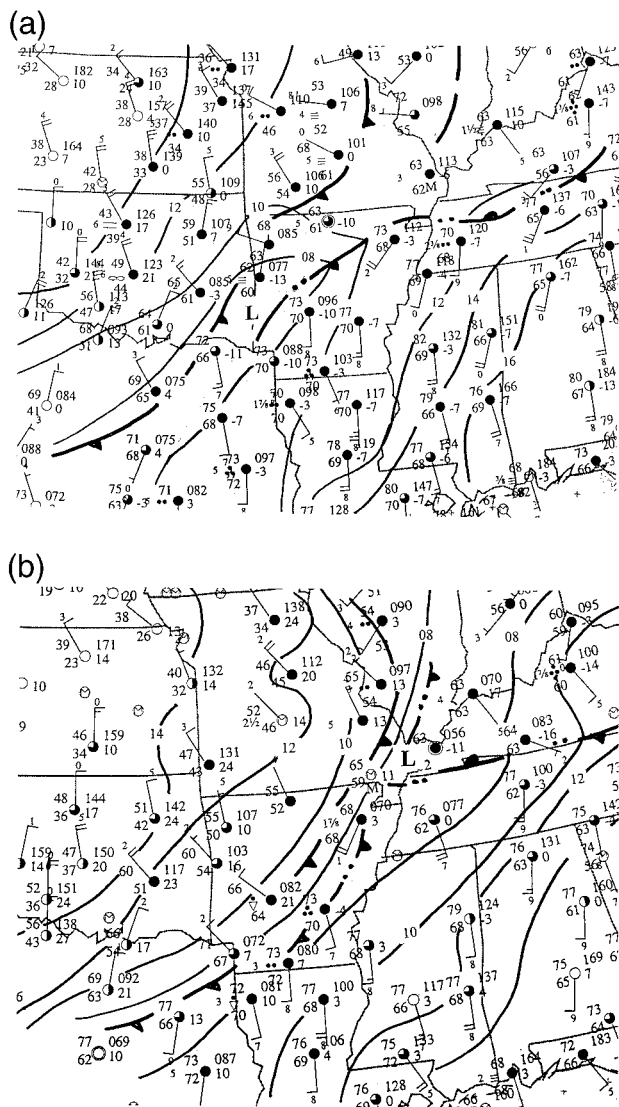
FIG. 9. Surface analysis for (a) 1800 UTC 1 Mar 1997 and (b) 0000 UTC 2 Mar 1997.
