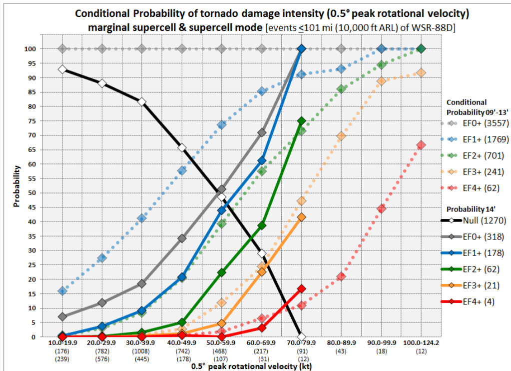
Figure 3. As in Fig. 2, but for 0.5^\circ peak V_{rot} (kt; x-coordinate).
