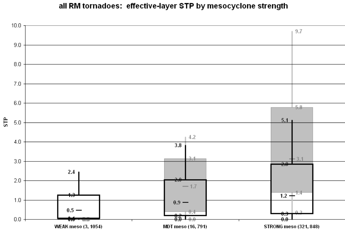
Figure 4. Effective-layer STP (dimensionless; sample period March 2005-December 2011) with all tornadic discrete right-moving supercells (RM) for weak, moderate (MDT), and strong mesocyclones. The shaded boxes (gray labels on the right) denote RM with EF3+ tornado damage, and the black overlays (with labels on the left) represent the RM that produced EF0 tornado damage. Sample sizes are denoted in parentheses (RM EF3+ tornadoes, RM EF0 tornadoes). The sample size for EF3+ tornadoes with weak mesocyclones was too small (3 cases) to justify a box and whisker plot. The shaded boxes span the 25th to the 75th percentiles with the median values marked within the box, and the whiskers extend upward to the 90th and downward to the 10th percentiles.
