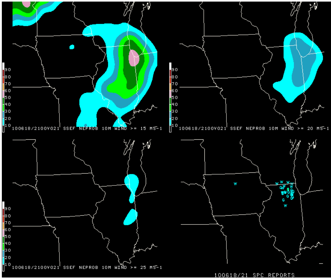
Figure 5. 21-hr SSEF forecasts of neighborhood exceedance probability of 10 m wind speeds \geq 30 \text{ kt} (upper left), \geq 40 \text{ kt} (upper right, and \geq 50 \text{ kt} (lower left) valid at 21 UTC 18 June 2010. Severe weather reports during the hour ending 21 UTC plotted in lower right, with “W” and “G” denoting locations of wind damage and severe wind gusts, respectively.
