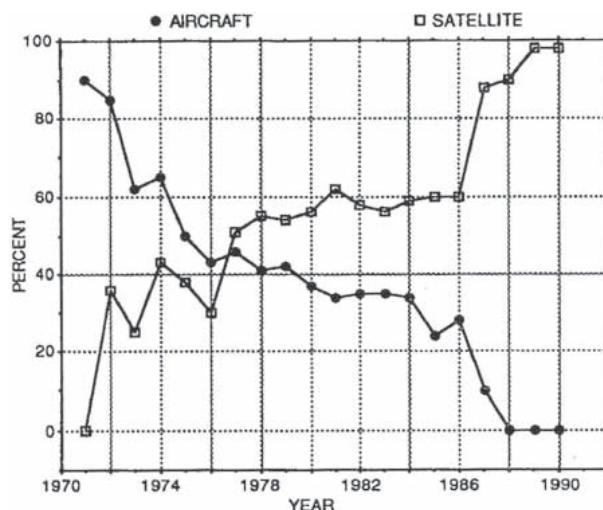
FIG. 6. Reconnaissance platforms used for JTWC warnings in the WestPac (from Guard et al. 1992).
