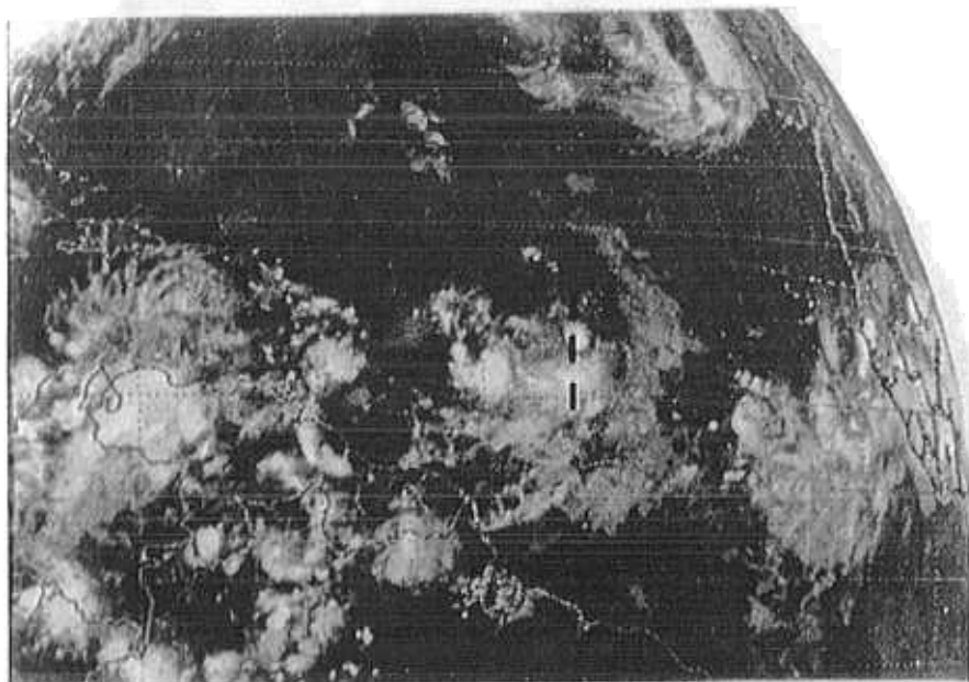
i) 0001 7 September 1988
