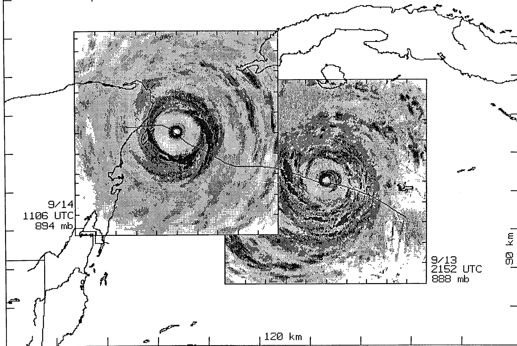
Fig. 14. Radar reflectivity pattern of Hurricane Gilbert near 1106 UTC September 14, and reflectivity pattern at 2152 UTC September 13, 1988. Light (dark) stippling represents light (heavy) rainfall. Figure provided by NOAA-AOML HRD.
