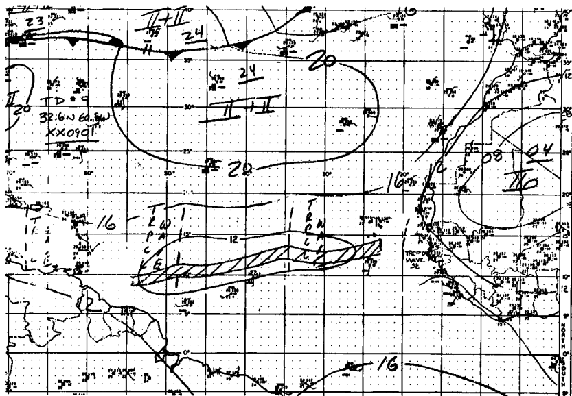
a) 0000 3 September 1988
