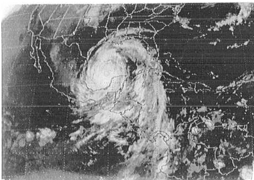
nn) 1201 15 September 1988
