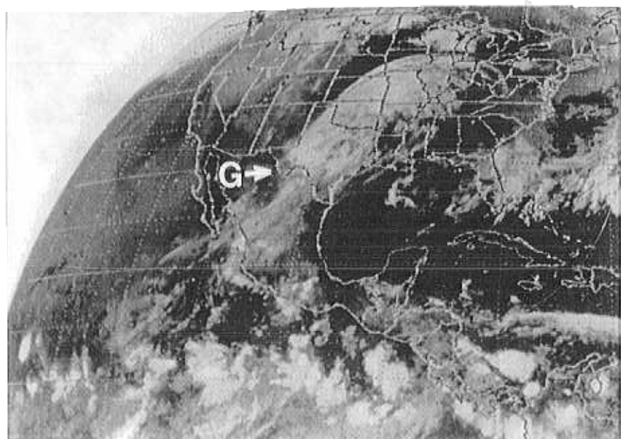
zz) 1201 18 September 1988
