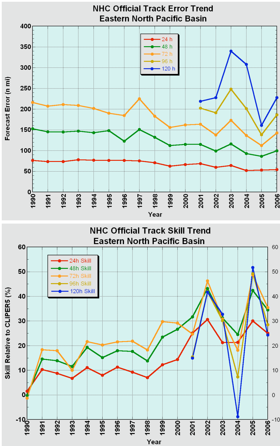
Figure 7. Recent trends in NHC official track forecast error (top) and skill (bottom) for the eastern North Pacific basin.
