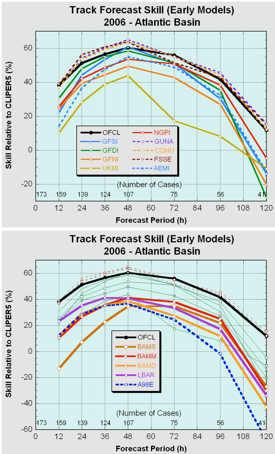
Figure. 2. Homogenous comparison for selected Atlantic basin early track guidance models for 2006. The top panel shows just the more advanced models (which also appear in the bottom panel as thin lines). Simpler models are highlighted in the bottom panel.
