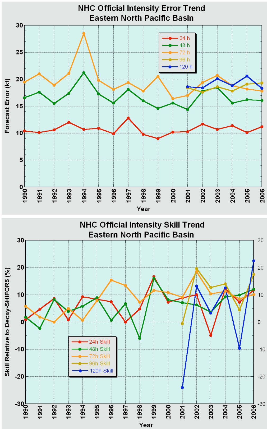
Figure 11. Recent trends in NHC official intensity forecast error (top) and skill (bottom) for the eastern North Pacific basin.
