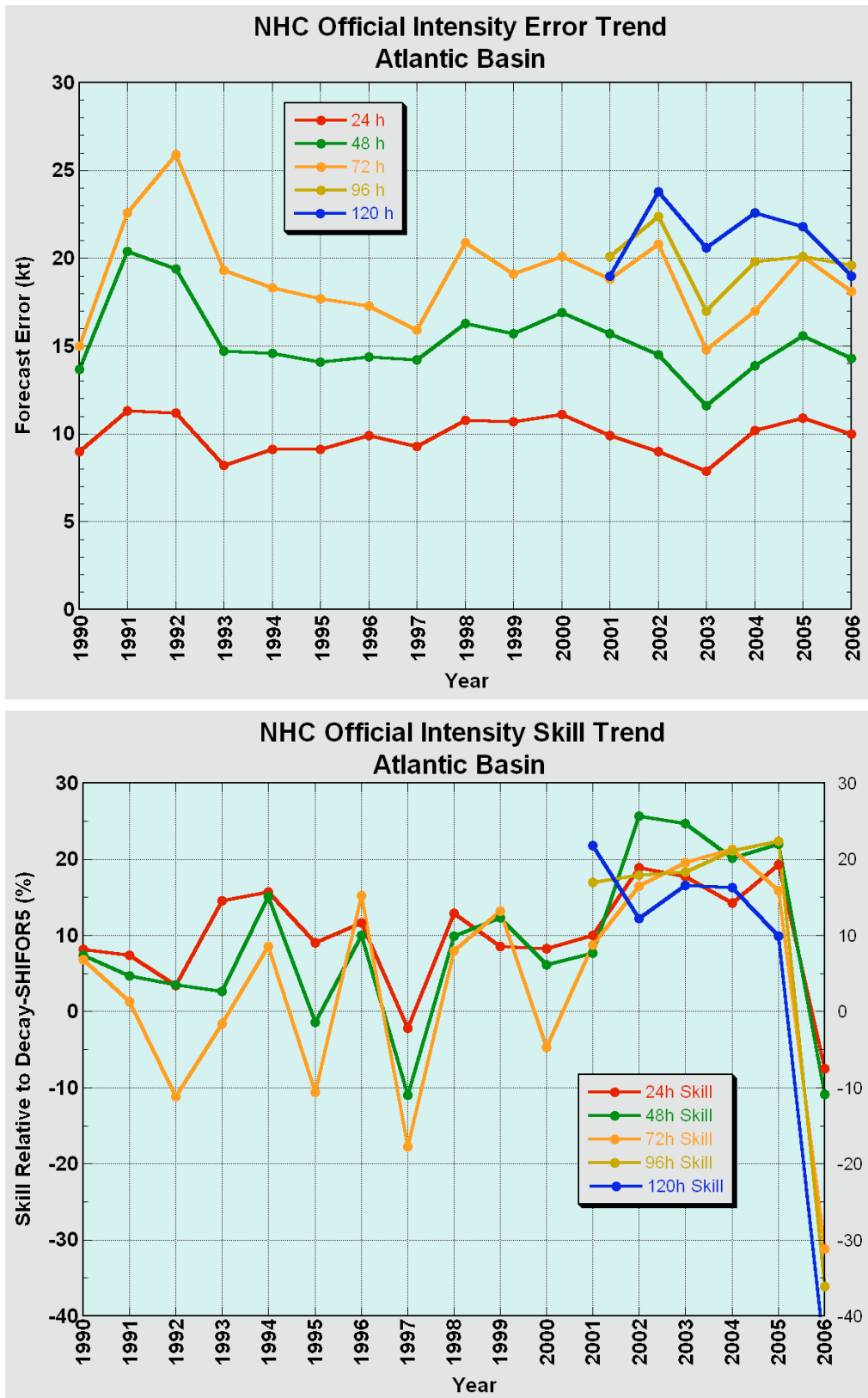
Figure 5. Recent trends in NHC official intensity forecast error (top) and skill (bottom) for the Atlantic basin.
