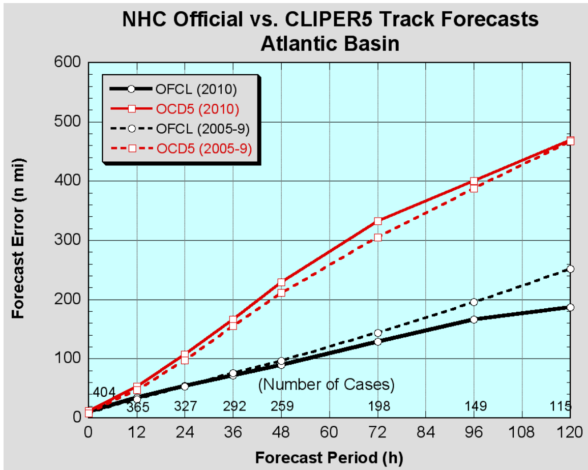
Figure 1. NHC official and CLIPER5 (OCD5) Atlantic basin average track errors for 2010 (solid lines) and 2005-2009 (dashed lines).
