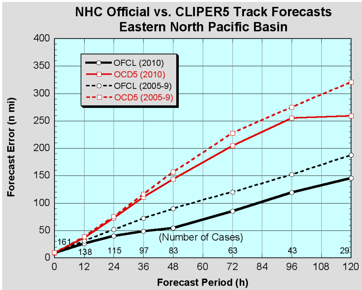
Figure 9. NHC official and CLIPER5 (OCD5) eastern North Pacific basin average track errors for 2010 (solid lines) and 2005-2009 (dashed lines).
