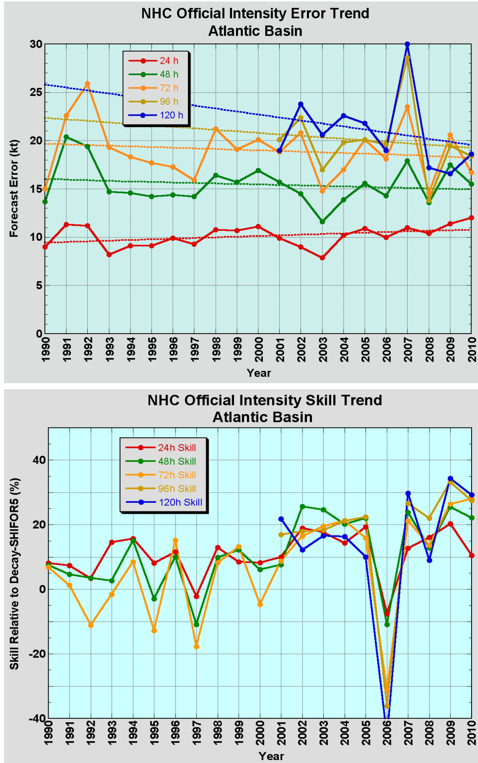
Figure 6. Recent trends in NHC official intensity forecast error (top) and skill (bottom) for the Atlantic basin.
