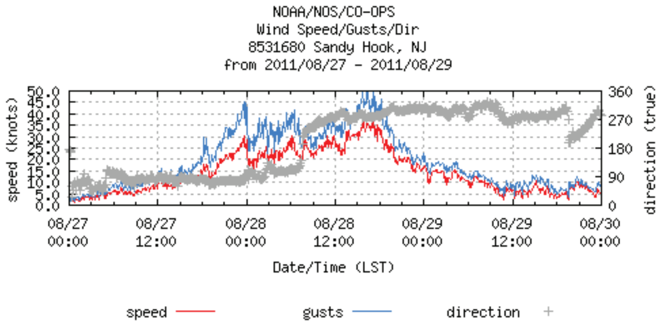
Fig.4. Wind speed, gust, and direction at Sandy Hook, NJ, during Irene.
