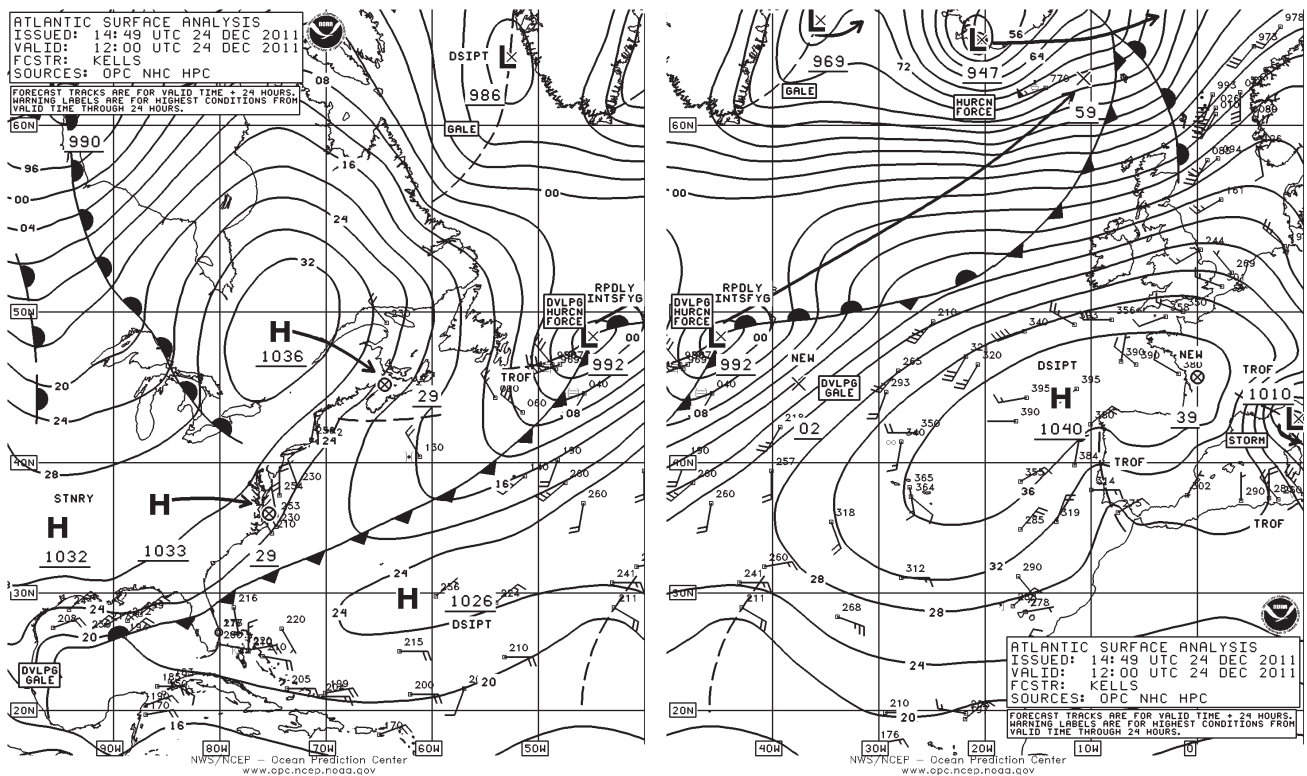
Figure 24. OPC North Atlantic Surface Analysis charts (Parts 1 and 2) valid 1200 UTC December 24, 2011.
