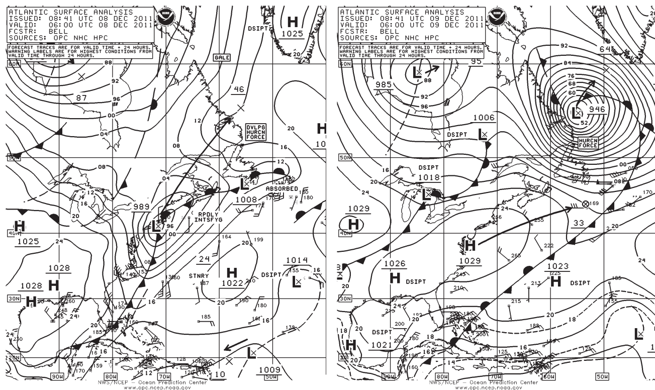
Figure 20. OPC North Atlantic Surface Analysis charts (Part 2) valid 0600 UTC December 8 and 9, 2011.
