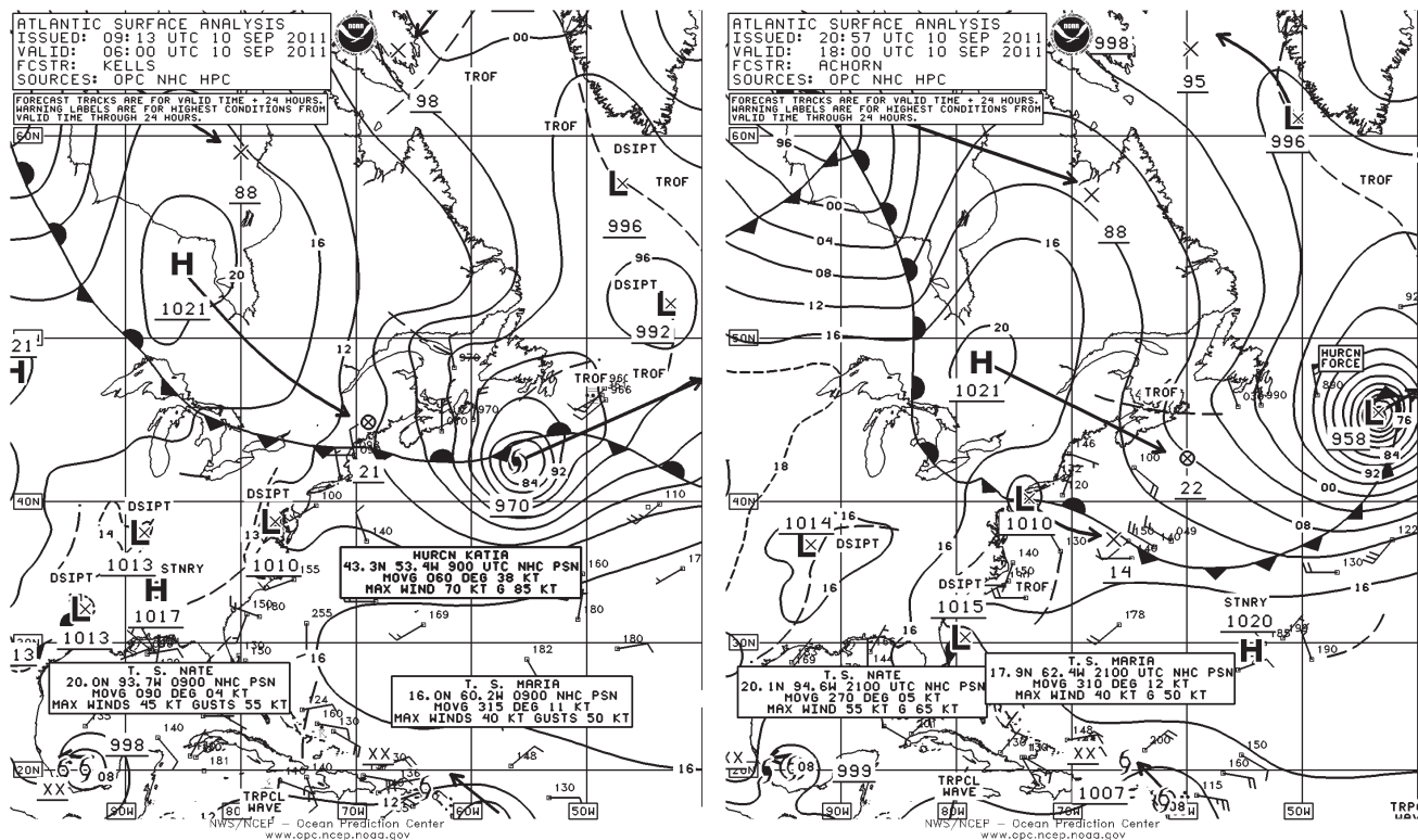
Figure 4. OPC North Atlantic Surface Analysis charts (Part 2) valid 0600 UTC and 1800 UTC September 10, 2011.
