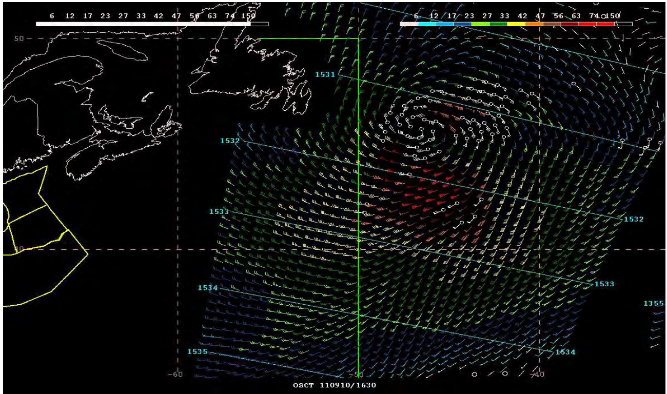
Figure 5. OSCAT (Indian scatterometer) image of satellite-sensed winds around Post-Tropical Katia with 50-km resolution.
