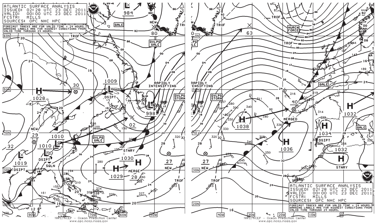
Figure 23. OPC North Atlantic Surface Analysis charts (Parts 1 and 2) valid 0000 UTC December 23, 2011.
