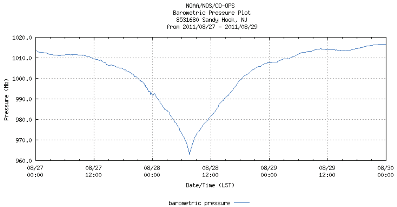
Fig.3. Barometric pressure measurement at Sandy Hook, NJ, during Irene.
