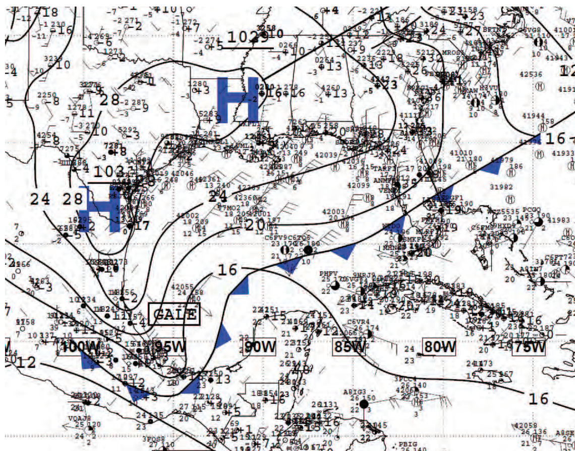
Figure 4. The NWS Unified Surface Analysis from 1200 UTC 25 Feb 12. A strong cold front followed by surface ridging building into the basin from the northwest produced a large area of gale force winds with several ship and buoy observations above 30 kts.
