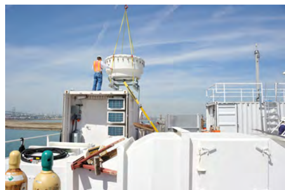
Unknown dock worker aligning radar being loaded on radar van on HORIZON SPIRIT. Photo: courtesy of Ernie R. Lewis, Lead investigator of MAGIC
