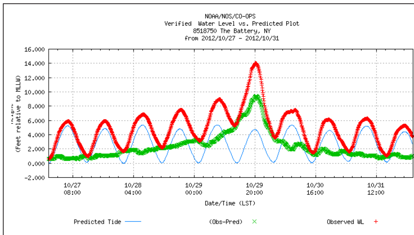
Figure 7. Water-level measurements at the Battery, NY during Sandy.
