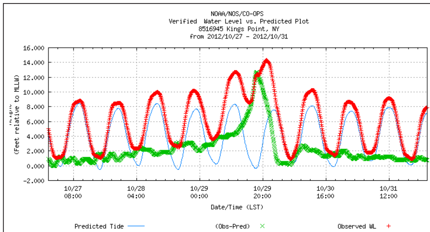
Figure 5. Water-level measurements at Kings Point, NY during Sandy. Storm surge is in green, storm tide is in red, and astronomical tide is in blue.
