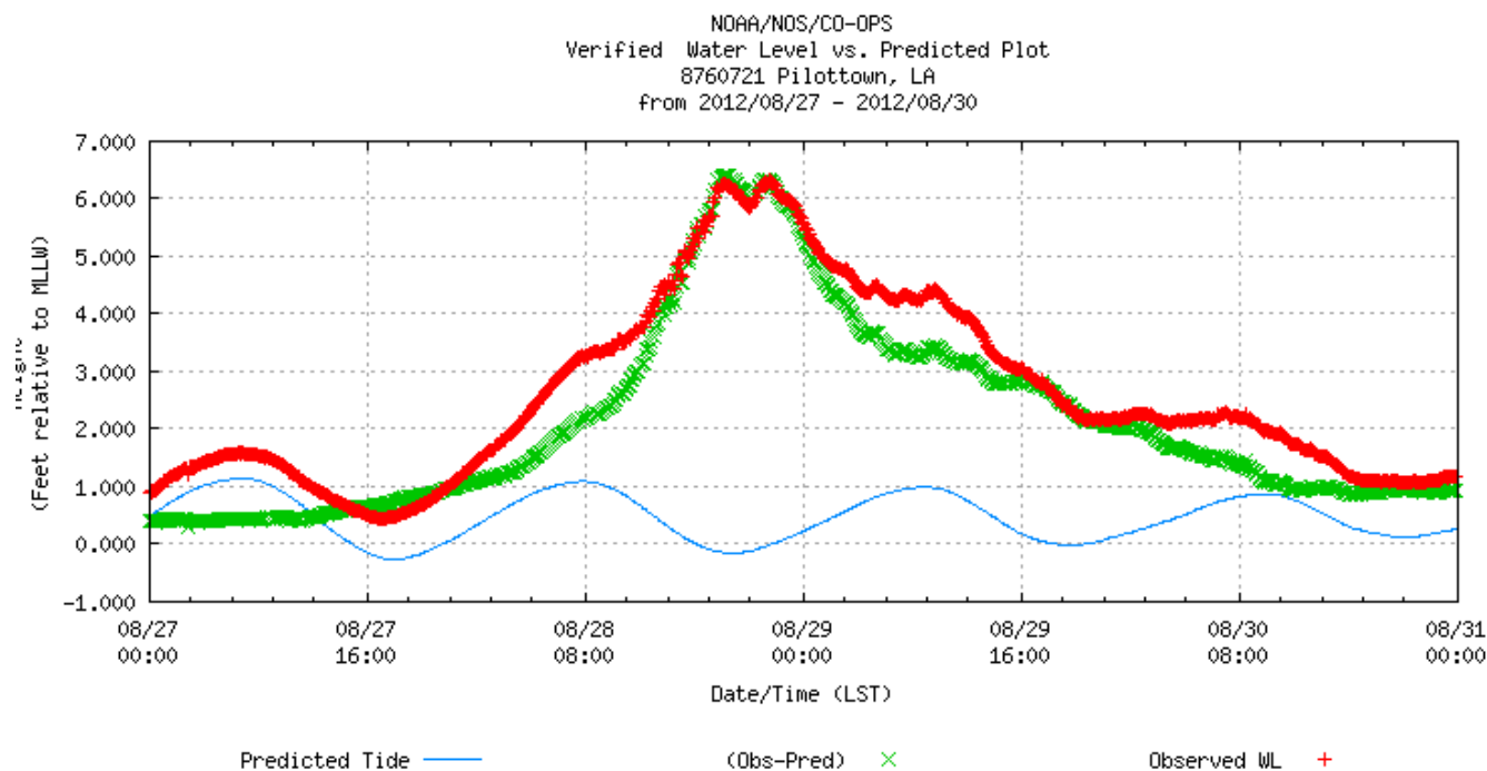
Fig. 5. Storm surge at PILL1 during Isaac.
