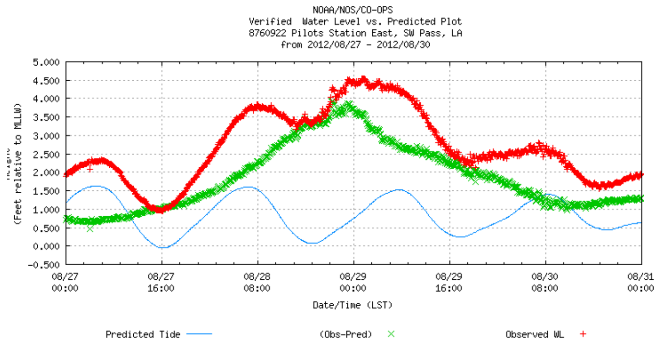
Fig.4. Storm surge at PSTL1 during Isaac.
