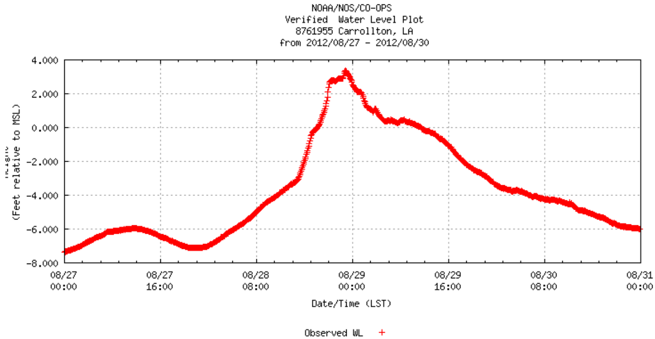
Fig.6. Storm surge at CARL1 during Isaac.
