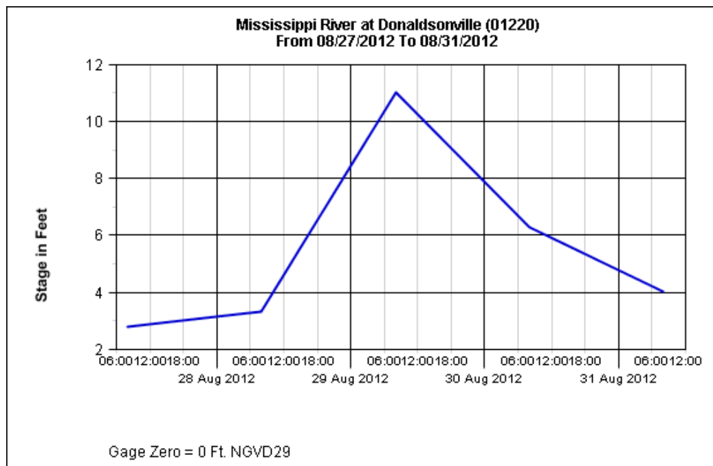
Fig.9. USACE measurements of the Mississippi River stage at Donaldsonville, LA during Isaac. Note that this station is located at 173.6 river miles upstream from the river mouth.
