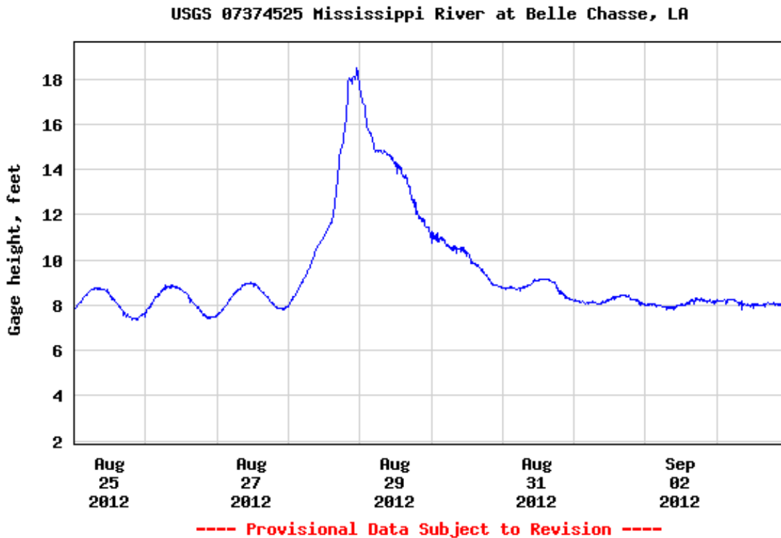
Fig.8. River stage at Belle Chase, LA, during Isaac based on USGS measurements.
