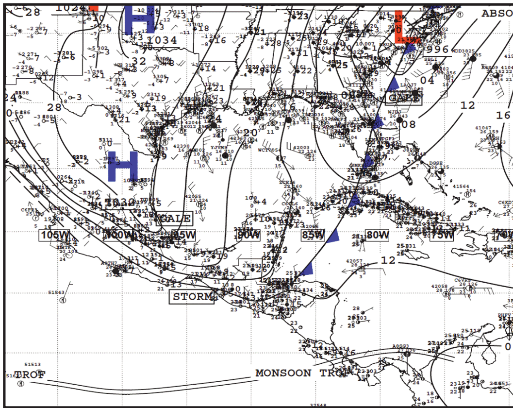
Figure 4. National Weather Service Unified Surface Analysis (USA) valid 1200 UTC 27 Nov 2013.
