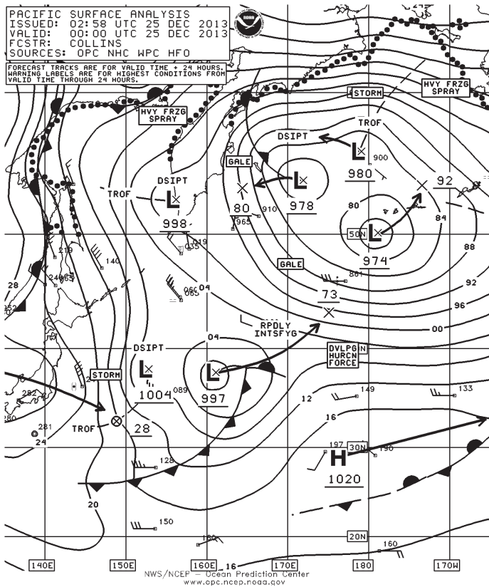
Figure 17. OPC North Pacific Surface Analysis charts (Part 2) valid 0000 UTC December 25 and 26, 2013.
