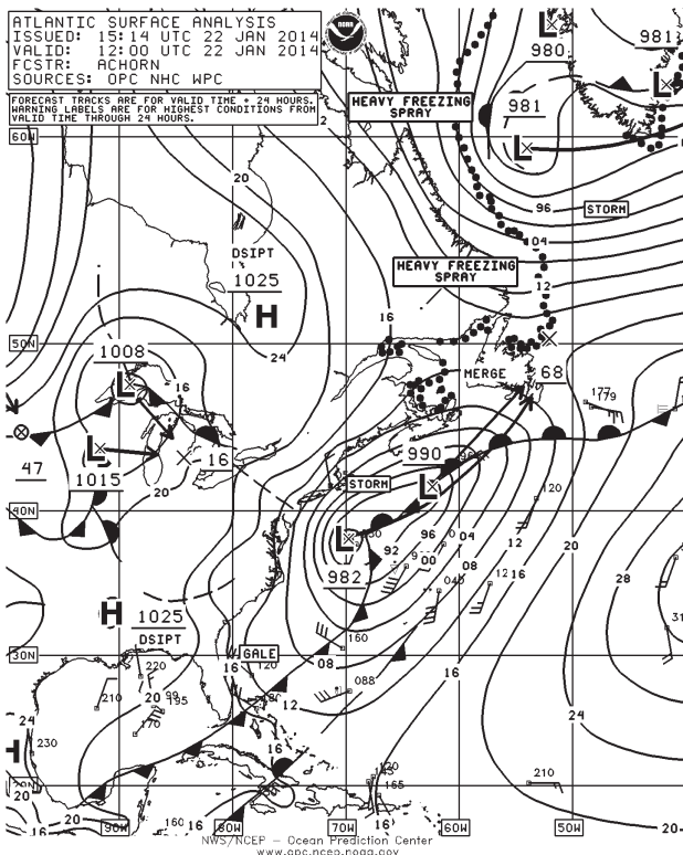
Figure 6. OPC North Atlantic Surface Analysis charts valid 1200 UTC January 22 (Part 2) and 0000 UTC January 24, 2014 (Part 1).
