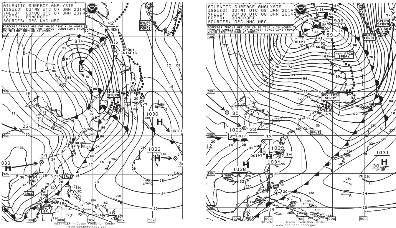
Figure 4. OPC North Atlantic Surface Analysis charts (Part 2) valid 0000 UTC January 7 and 8, 2014.
