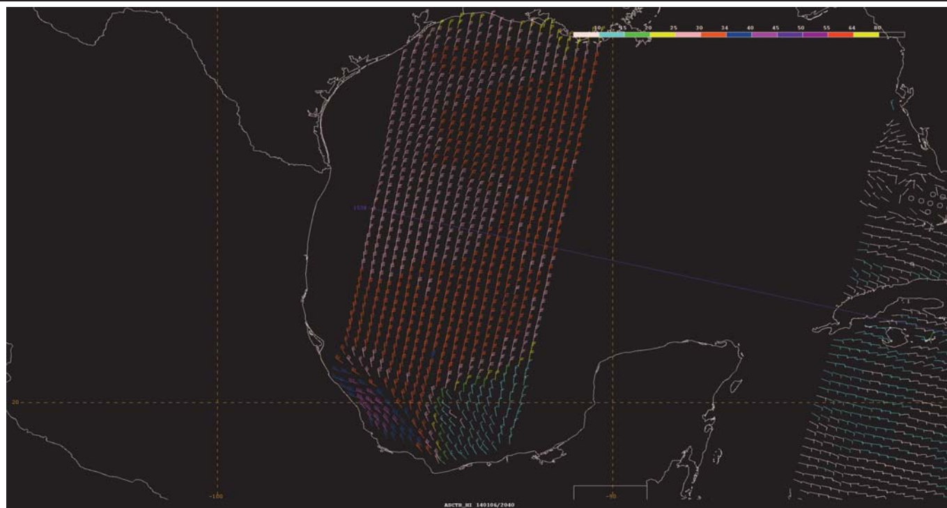
Figure 2. A scatterometer pass from the MetOp Advanced SCATerometer (ASCAT-B) valid around 1538 UTC 06 January. Note the dark blue and pink wind barbs in the southwestern Gulf of Mexico indicating gale force winds between 34 kts and 45 kts.
