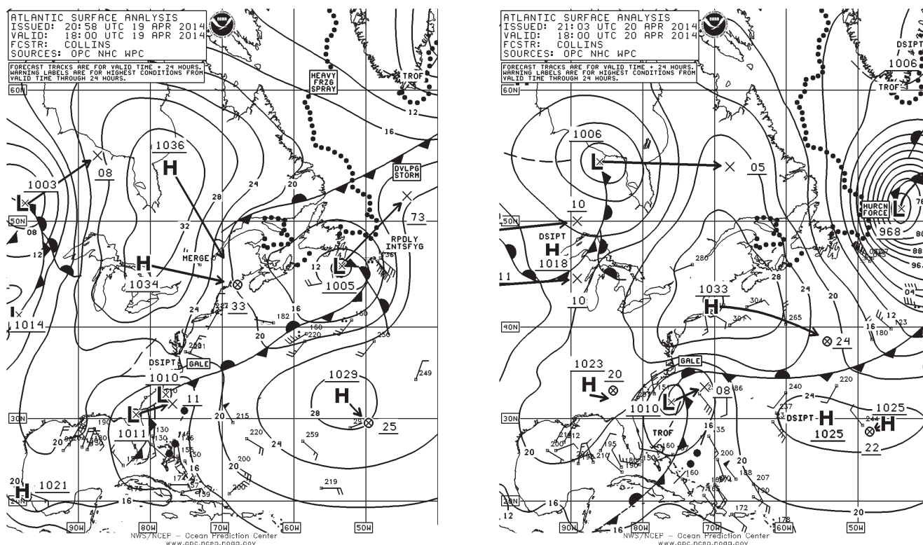
Figure 24. OPC North Atlantic Surface Analysis charts (Part 2) valid 1800 UTC April 19 and 20, 2014.
