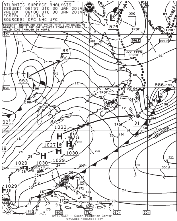
Figure 8. OPC North Atlantic Surface Analysis charts valid 0600 UTC January 30 (Part 2) and 1800 UTC January 31, 2014.
