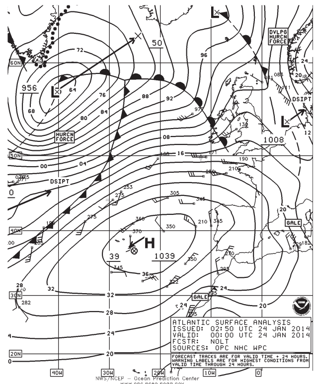
Figure 6. OPC North Atlantic Surface Analysis charts valid 1200 UTC January 22 (Part 2) and 0000 UTC January 24, 2014 (Part 1).
