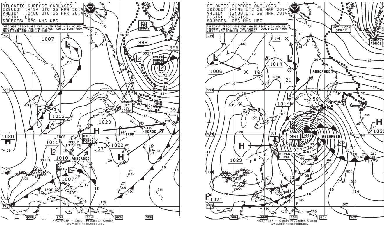
Figure 21. OPC North Atlantic Surface Analysis charts (Part 2) valid 1200 UTC March 25 and 26, 2014.
