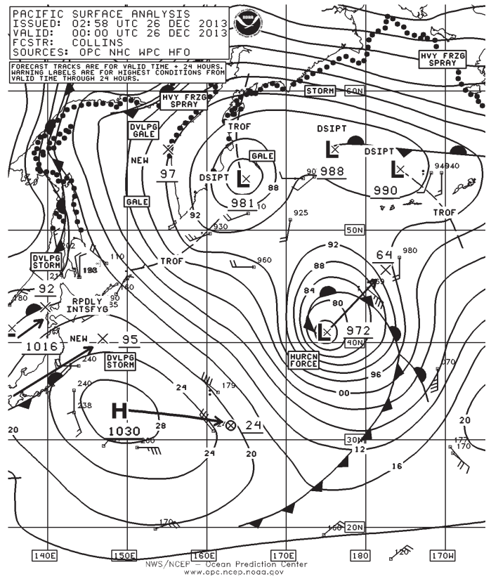
Figure 17. OPC North Pacific Surface Analysis charts (Part 2) valid 0000 UTC December 25 and 26, 2013.
