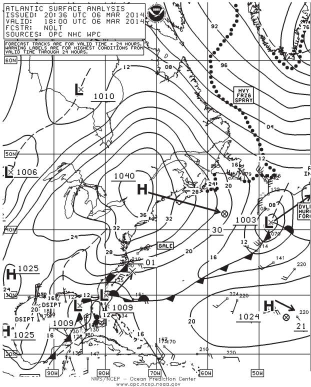
Figure 20. OPC North Atlantic Surface Analysis charts valid 1800 UTC March 6 (Part 2) and 1800 UTC March 7, 2014 (Part 1).
