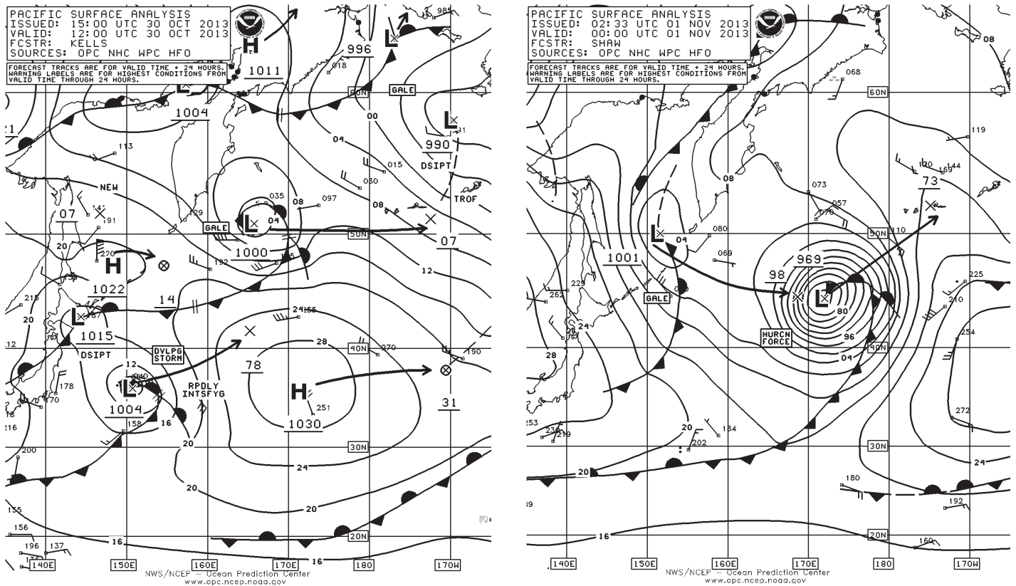
Figure 10. OPC North Pacific Surface Analysis charts (Part 2) valid 1200 UTC October 30 and 0000 UTC November 1, 2013.
