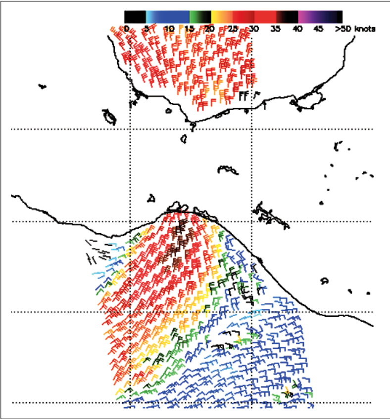
Figure 7. European Advanced Scatterometer (ASCAT A) pass valid at 0400 UTC 23 November 2015. Note the 40-45 kts wind barbs south of the Gulf of Tehuantepec near 15N95W.
