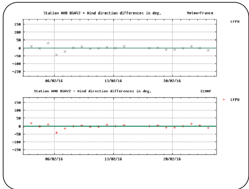
Intercomparison with reference models has proven the good quality of the data, here e.g. wind direction.
