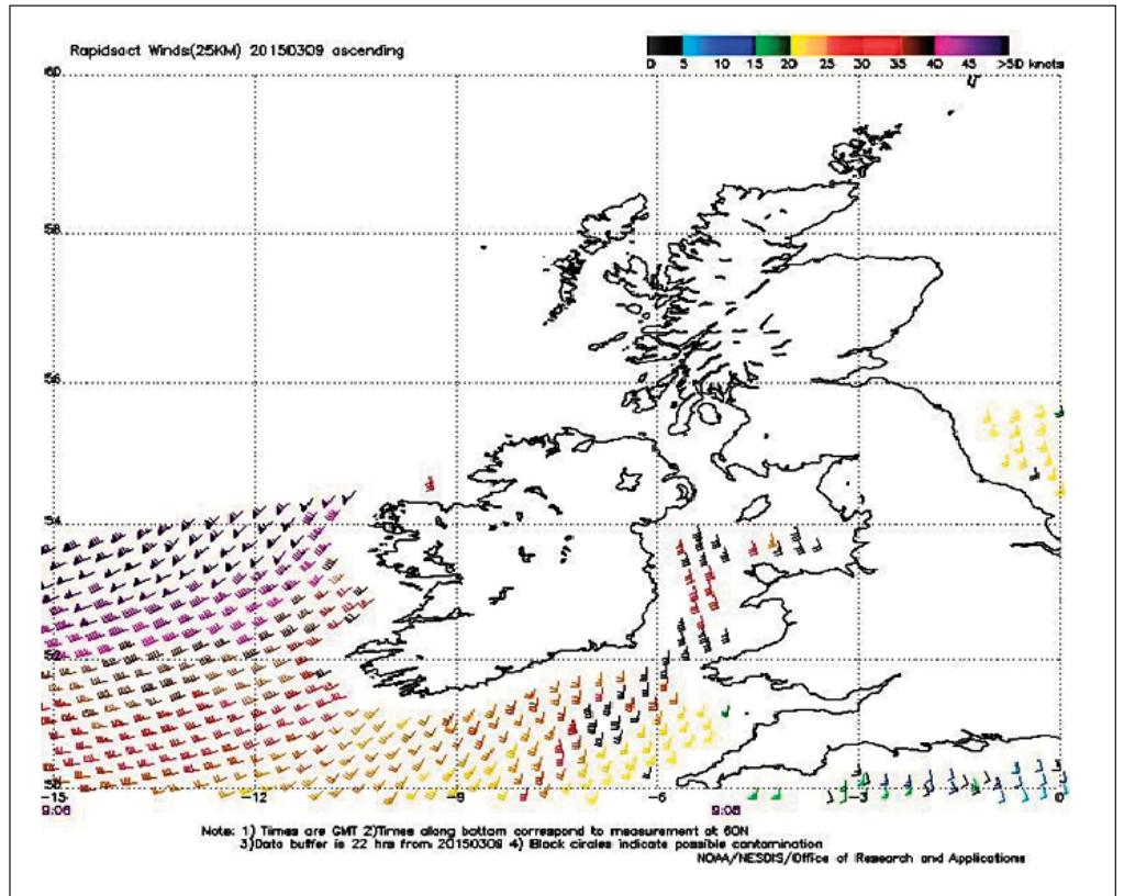
Figure 9. Rapidscat image of remotely-sensed winds from an instrument aboard the International Space Station with resolution of 25 km, for the same cyclone as shown in Figure 6.
