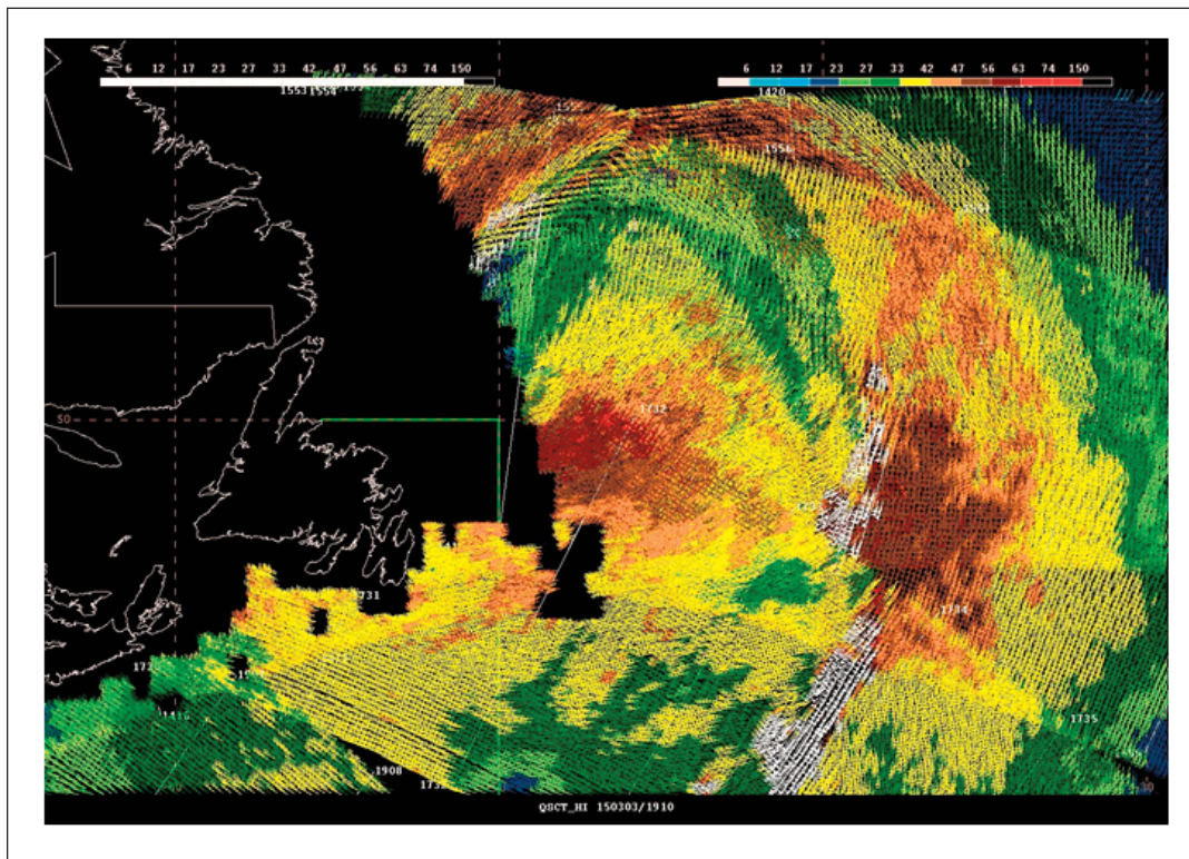
Figure 2. RapidScat image of remotely-sensed winds from an instrument aboard the International Space Station with resolution of 12.5 km. Wind barbs are colored according to a scale on the upper right side of the image. Diagonal lines are cross-track timelines of the instrument labeled in UTC. The line crossing the center of the image where the highest winds are found is for 1732 UTC March 3, 2015, or six and one-half hours prior to the valid time of the second part of Figure 1. Imagery is courtesy of NOAA/NESDIS/STAR (Center for Satellite Applications and Research).
