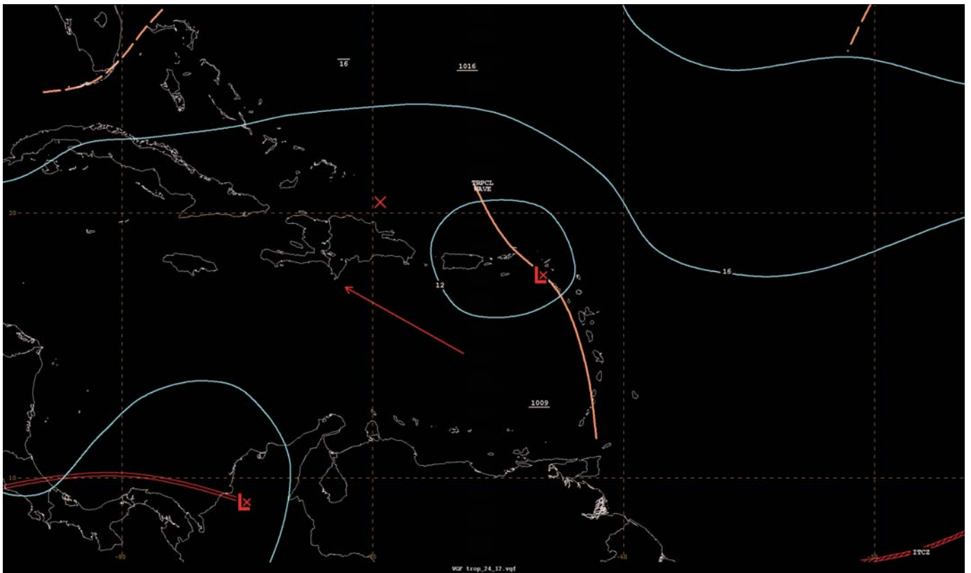
Figure 9. National Weather Service Unified Surface Analysis (USA) from 1200 UTC 24 Aug. Note the close spacing between the 1012 hPa and 1016 hPa isobars.
