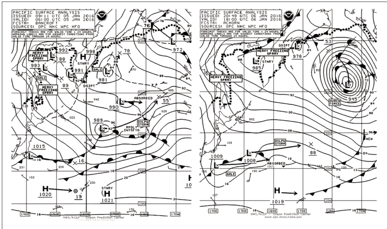
Figure 3. OPC North Pacific Surface Analysis charts (Part 2) valid 0600 UTC January 5 and 1800 UTC January 6, 2016.
