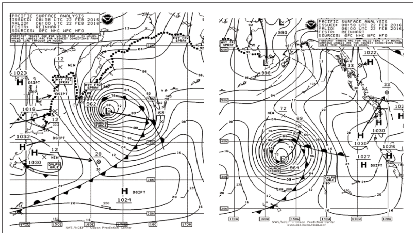
Figure 19. OPC North Pacific Surface Analysis chart (Parts 2 and 1) valid 0600 UTC February 22, 2016.
