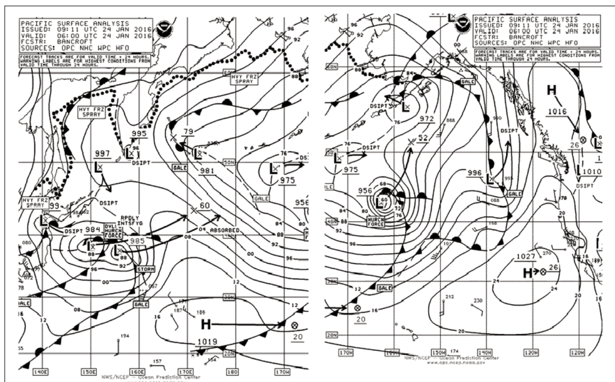
Figure 11. OPC North Pacific Surface Analysis chart (Parts 2 – west and 1 – east) valid 0600 UTC January 24, 2016. The two parts overlap between 165W and 175W.
