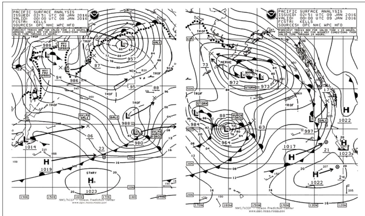
Figure 4. OPC North Pacific Surface Analysis charts valid 0000 UTC January 8 (Part 2) and 0000 UTC January 9, 2016 (Part 1).
