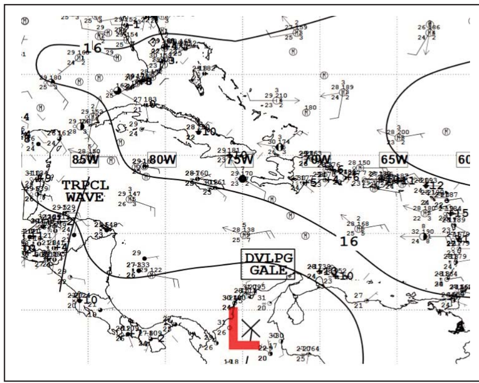
Figure 6.- National Weather Service Unified Surface Analysis (USA) from 0000 UTC 17 Jun. Note the tight gradient spacing just north of the coasts of Colombia and Venezuela between the 1016 hPa and 1012 hPa isobars.
