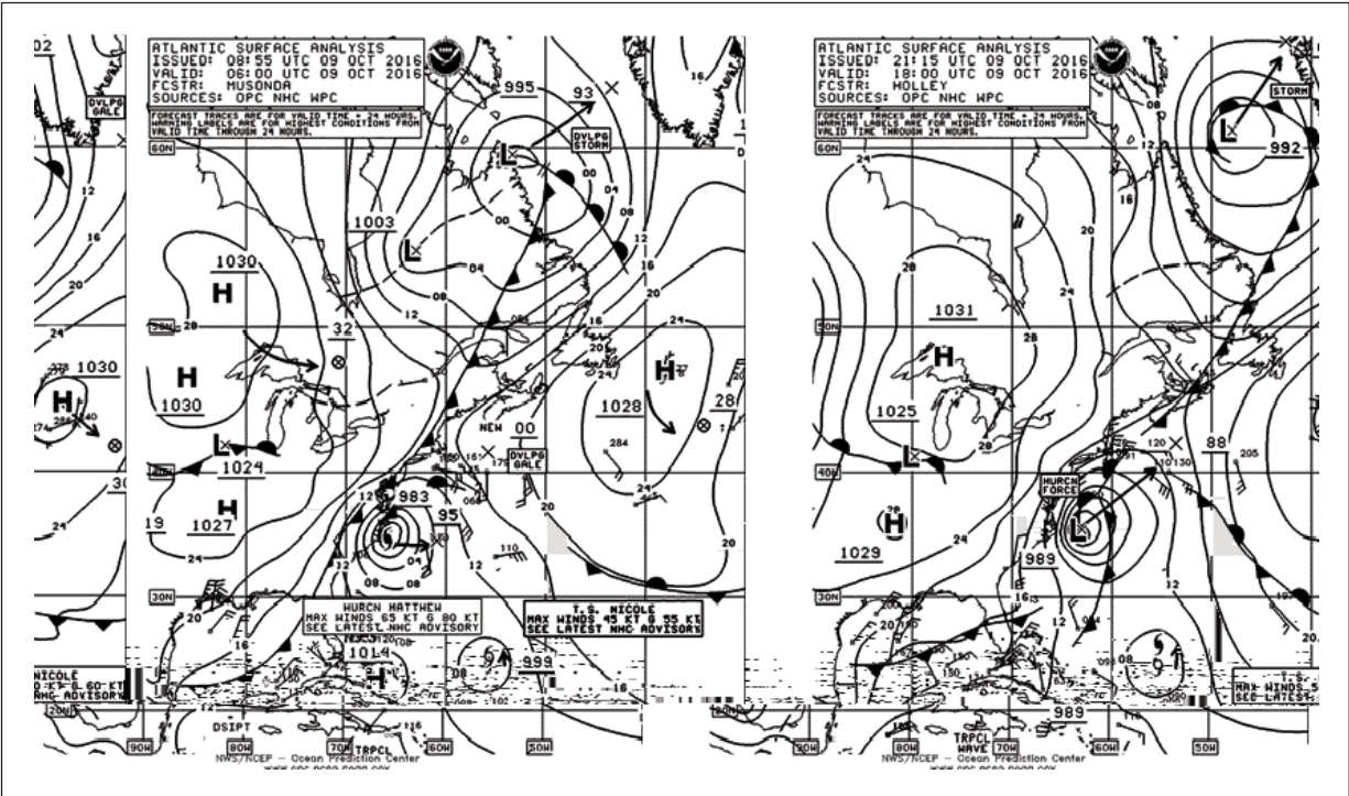
Figure 5. OPC North Atlantic Surface Analysis Charts (Part 2) valid 0600 and 1800 UTC October 9, 2016.
