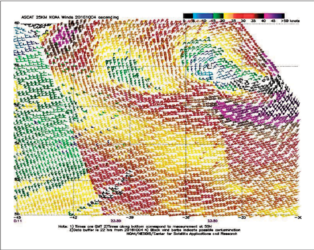
Figure 15. ASCAT (METOP-A) image of satellite-sensed winds with 25-km resolution around the hurricane-force low shown in the second part of Figure 14 . The pass containing the stronger wind retrievals has a valid time of 2350 UTC October 4, 2016, or about 6 hours later than the valid time of the second part of Figure 14 . The southern tip of Greenland appears near the upper left corner of the image. Imagery is courtesy of OAA/NESDIS/Center for Satellite Applications and Research.
