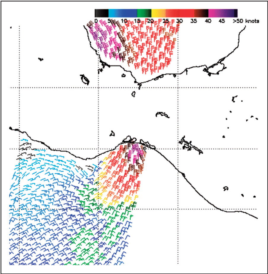
Figure 2. A scatterometer pass from the MetOp Advanced Scatterometer (ASCAT-A) valid around 1629 UTC 07 January. Note the magenta wind barbs over the Gulf of Tehuantepec indicating gale-force winds between 40 kts and 45 kts.
