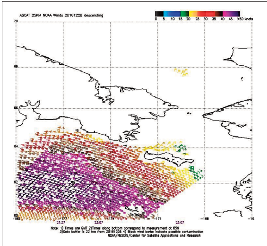
Figure 33. ASCAT (METOP-A) image of satellite-sensed winds (25-km resolution) on the northeast side of the large hurricane-force system shown in the second part of Figure 31 . Portions of two passes are shown, with the valid time of the later pass (2307 UTC December 28, 2016) about 1 hour prior to the valid time of the second part of Figure 31 . Image is courtesy of NOAA/NESDIS/Center for Satellite Application and Research.
