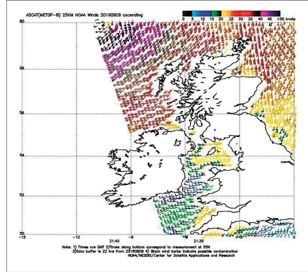
Figure 9. ASCAT (METOP-B) image of satellite-sensed winds with 25-km resolution around the southeast side of the cyclone northwest of the British Isles shown in the second part of Figure 8 . The valid time of the pass is 2140 UTC September 9, 2016, or about 8.25 hours prior to the valid time of the second part of Figure 8 . Imagery is courtesy of NOAA/NESDIS/Center for Satellite Applications and Research.
