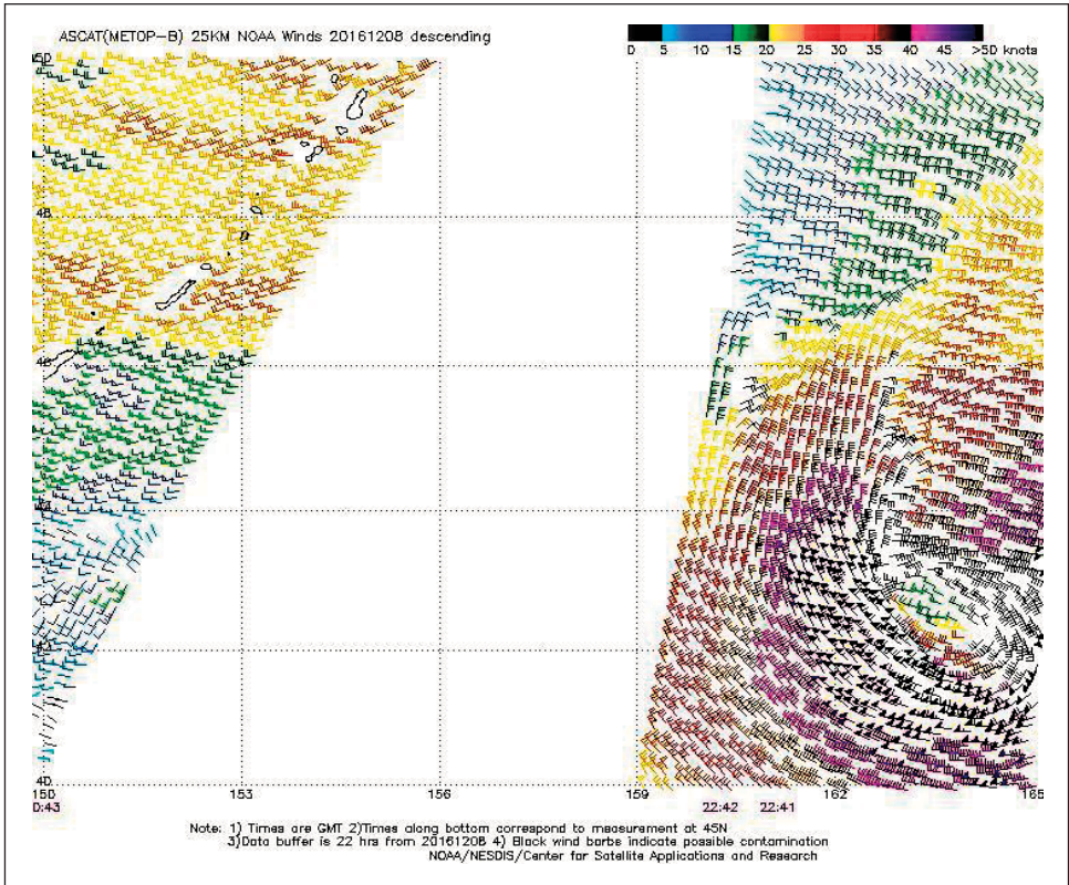
Figure 26. ASCAT (METOP-B) image of satellite-sensed winds (25-km resolution) around the hurricane-force low shown in the second part of Figure 25. The valid time of the pass containing the higher wind retrievals is 2241 UTC December 8, 2016, or about 1.25 hours prior to the valid time of the second part of Figure 25. A portion of the Kurile Islands appears on the upper left side of the image. Image is courtesy of NOAA/NESDIS/Center for Satellite Application and Research.
