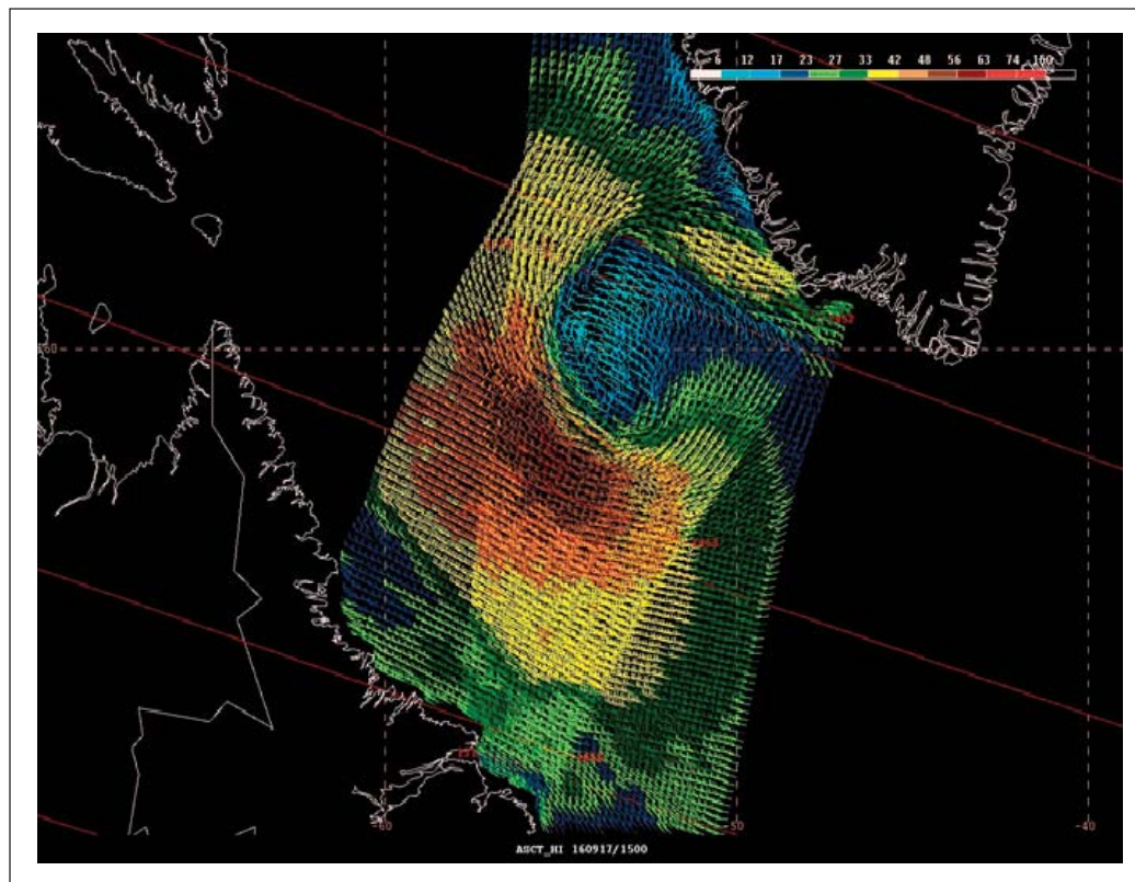
Figure 11. ASCAT (METOP-A) image of satellite-sensed winds with 25-km resolution around the storm shown in the second part of Figure 10 . The red lines labeled with four-digit UTC times are cross-track time lines of the satellite, with the higher wind retrievals in the lower-middle portion of the image in a pass corresponding to a valid time of 1453 UTC September 17, 2016, about 3 hours prior to the valid time of the second part of Figure 10 . Wind barbs are colored according to the scale near the top of the image. Imagery is courtesy of NOAA/NESDIS/Center for Satellite Applications and Research, adapted for operational use on OPC workstations.
