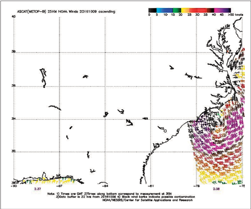
Figure 6. ASCAT METOP-B (Advanced Scatterometer) image of satellite-sensed winds with 25-km resolution around Hurricane Matthew shown in the first part of Figure 5 . The valid time of the pass is 0238 UTC October 9, 2016, or about 3.5 hours prior to the valid time of the first part of Figure 5 . Imagery is courtesy of NOAA/NESDIS/Center for Satellite Applications and Research.
