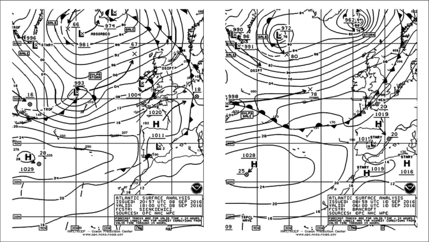
Figure 8. OPC North Atlantic Surface Analysis Charts (Part 1) valid 1800 UTC September 8 and 0600 UTC September 10, 2016.
