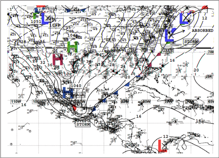
Figure 1. Unified Surface Analysis issued by the Ocean Prediction Center (OPC), the Weather Prediction Center (WPC), and the Tropical Analysis and Forecast Branch (TAFB) valid 1800 UTC 07 January 2017. The cold front over southeastern Mexico has already reached the Chivela Pass, with a 1044-hPa high centered over Texas and strong ridging nosing southward along eastern Mexico.
