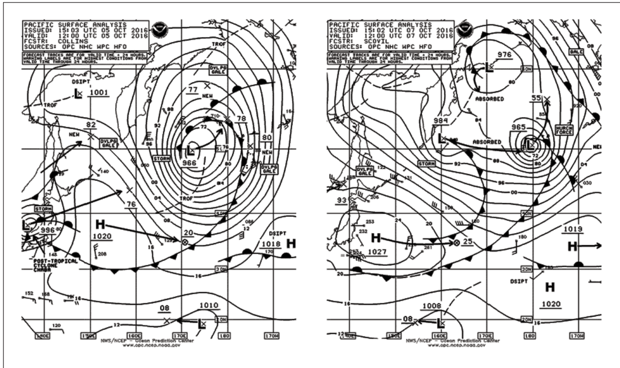
Figure 2. OPC North Pacific Surface Analysis Charts (Part 2 — West) valid 1200 UTC October 5 and 7, 2016.
