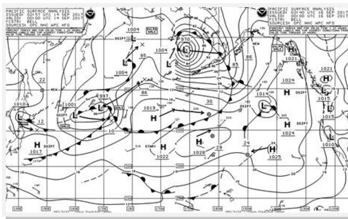
Figure 8. OPC North Pacific Surface Analysis charts valid 0000 UTC September 14 (Part 2) and 0000 UTC September 16, 2017 (Part 1).
