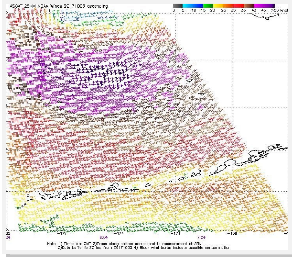
Figure 11. This is a 25-km ASCAT (METOP-A) image of satellite-sensed winds around the south side of the storm depicted in the second part of Figure 10. Portions of two passes are shown (0724 UTC and 0904 UTC October 5, 2017). The valid time of the later pass containing the highest wind retrievals is about 3 hours later than the valid time of the second part of Figure 10. Image is courtesy of NOAA/ NESDIS/ Center for Satellite Application and Research.
