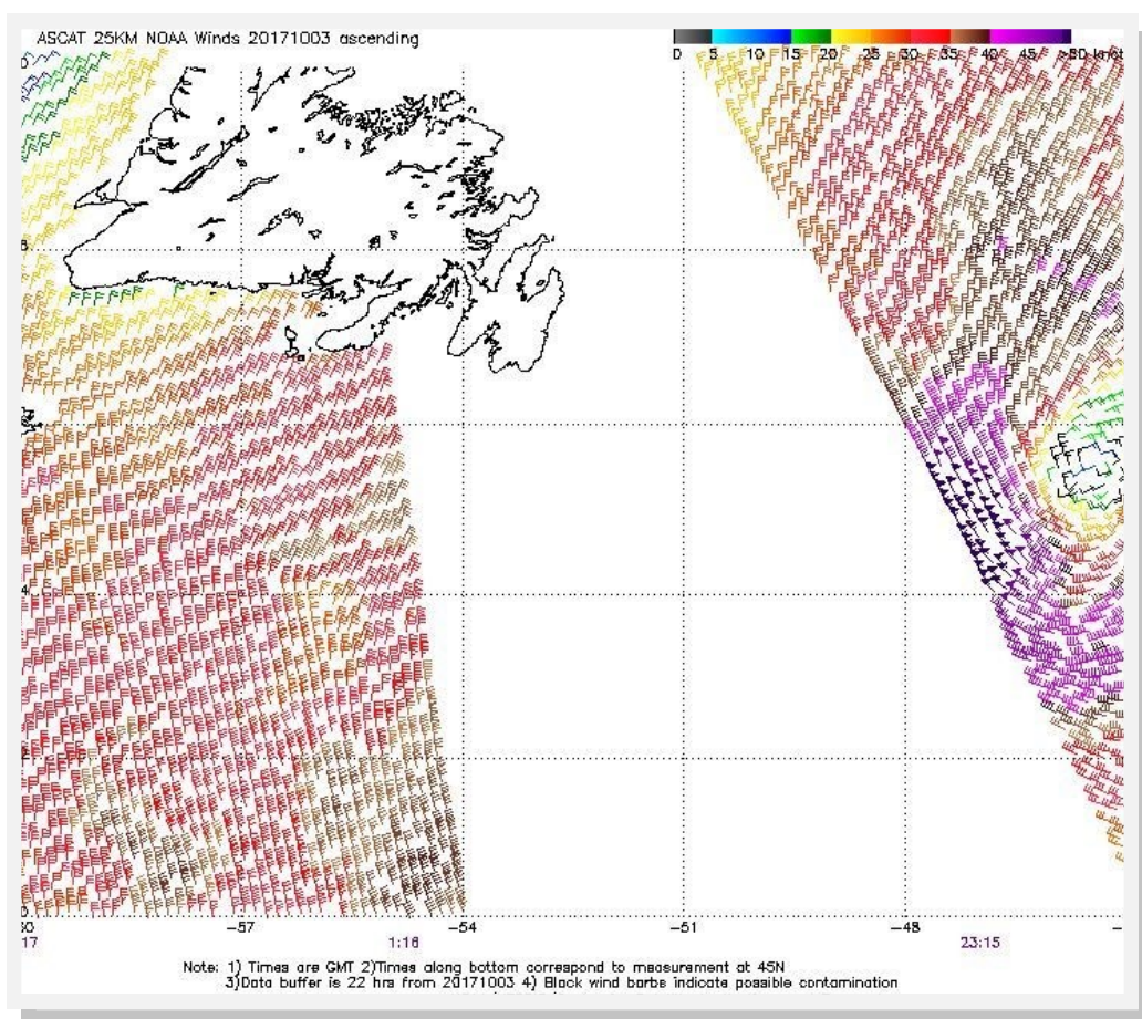
Figure 10. ASCAT (METOP-A) image of satellite-sensed winds with 25-km resolution around the south, west, and north sides of the storm shown in the second part of Figure 9. The valid time of the pass is 2315 UTC October 3, 2017, or 0.75 hour prior to the valid time of the second part of Figure 9. Imagery is courtesy of NOAA/NESDIS/ Center for Satellite Applications and Research.
