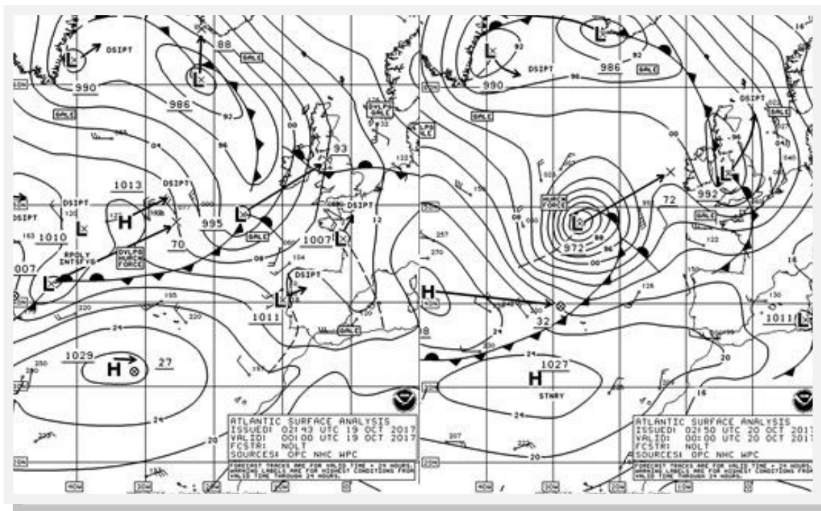
Figure 11. OPC North Atlantic Surface Analysis charts (Part 1) valid 0000 UTC October 19 and 20, 2017.
