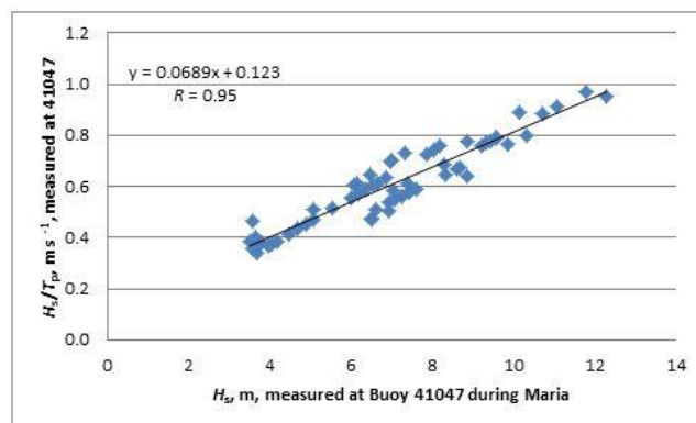
Figure 6. Relation between H_s and H_s/T_p at 41047 during Maria.
