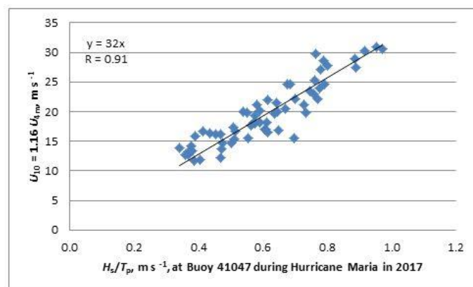
Figure 5. Relation between U_{10} and H_s/T_p at 41047 during Maria.
