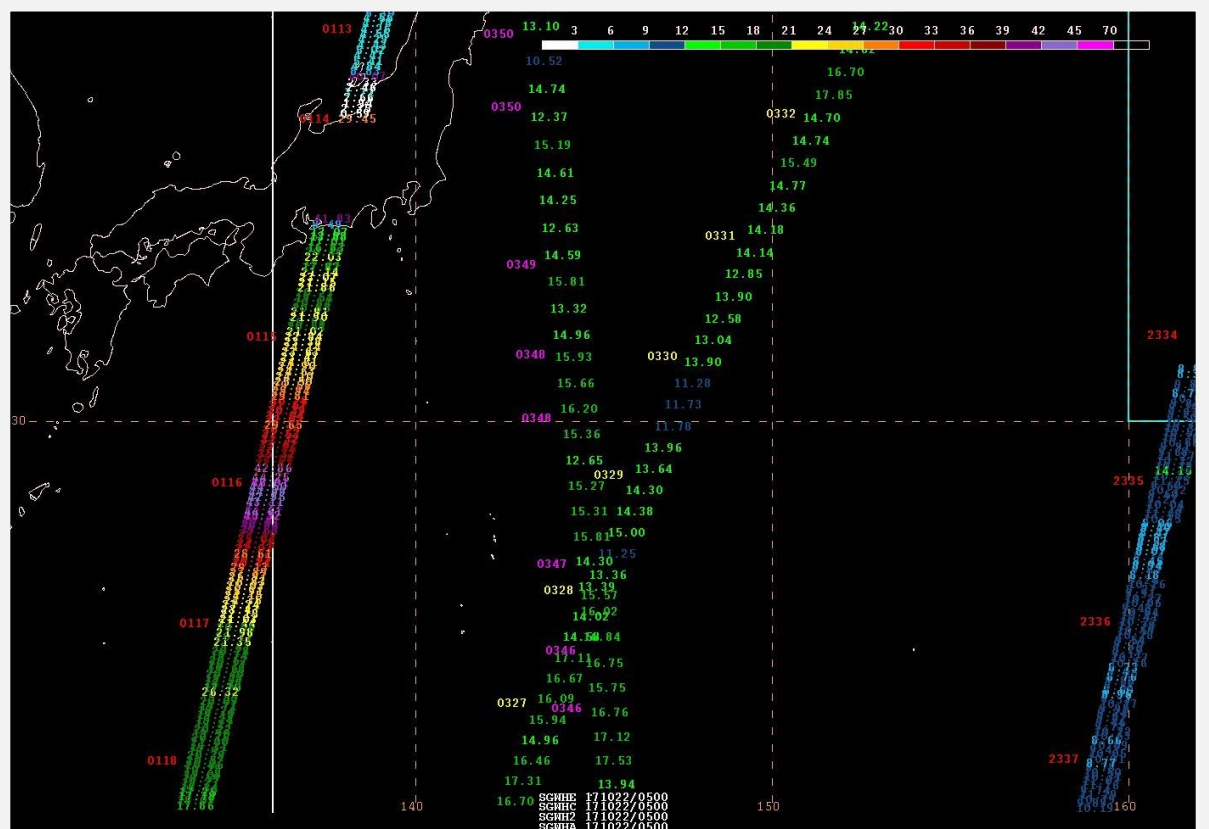
Figure 4. Altimeter pass from the AltiKa satellite with remotely sensed significant wave heights through Typhoon Lan south of Japan valid at 0116 UTC October 22, 2017. Wave heights in feet are given to two decimal places with satellite overpass times shown to the left in UTC. The color scale appears for the wave heights. Image is courtesy of NOAA/NESDIS/ Center for Satellite Application and Research, adapted for operational use at OPC.
