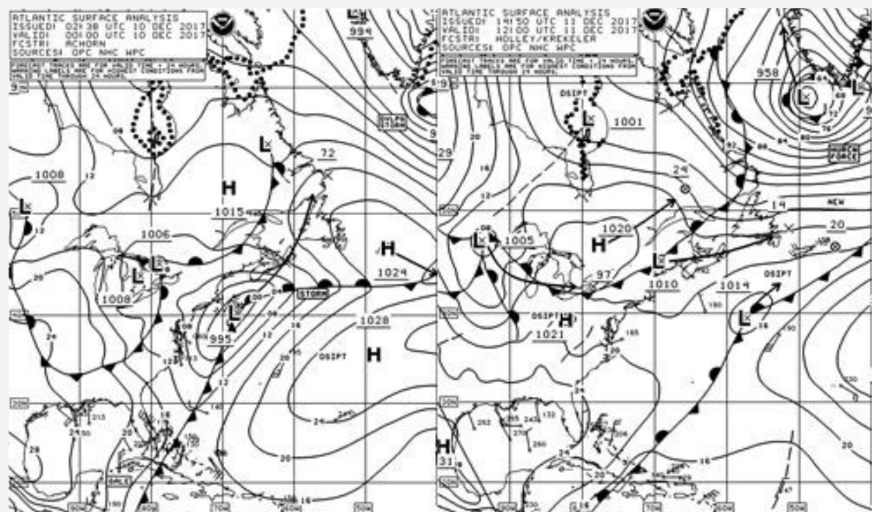
Figure 23. OPC North Atlantic Surface Analysis charts (Part 2) valid 0000 UTC December 10 and 1200 UTC December 11, 2017.
