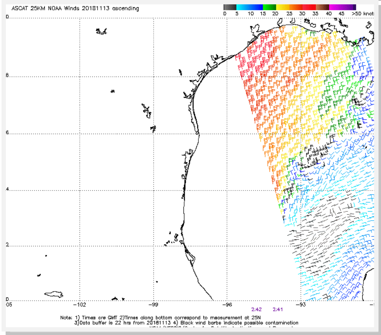
Figure 1. European Advanced Scatterometer (ASCAT A) Wind Vectors (kts) Valid 0241 UTC 13 Nov.
