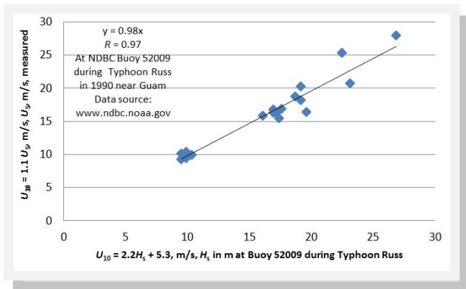
Figure 5. Verifying Equation (3) at the NDBC Buoy 52009 during Typhoon Russ in 1990.
