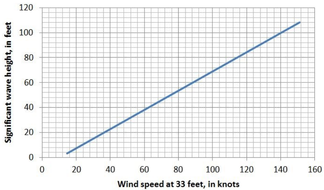
Figure 9. A Graph between Significant Wave Height and the Wind Speed (in British units).
