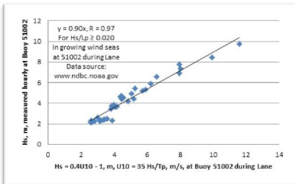
Figure 3. Validating Equation (2) at Buoy 51002 near Hawaii during Hurricane Lane in 2018.
