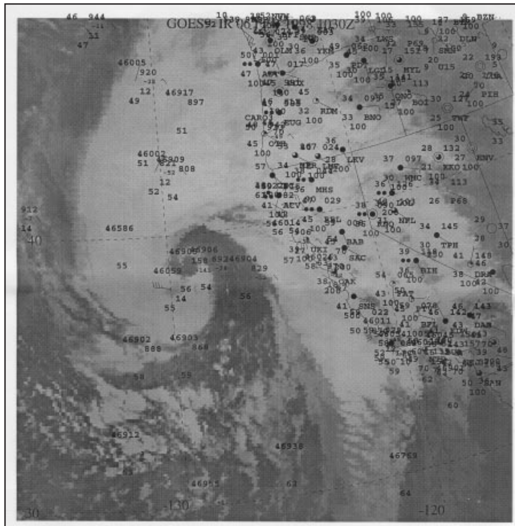
Figure 6. GOES-9 infrared satellite image of storm at 1030Z February 6 off California coast with plotted data
