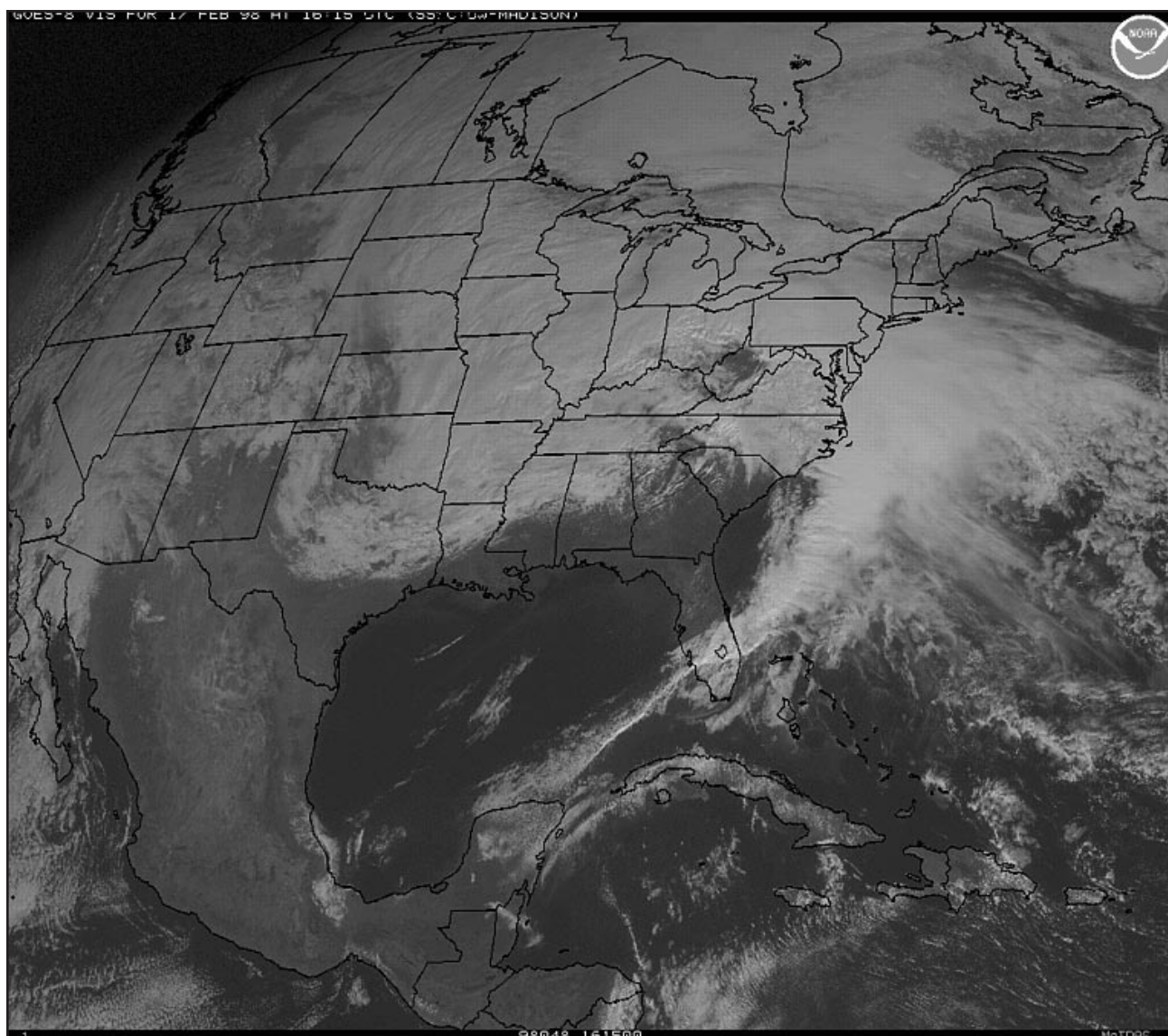
Figure 4. GOES-8 visible image at 1615 UTC 17 February 1998. Image courtesy of the National Climatic Data Center.
