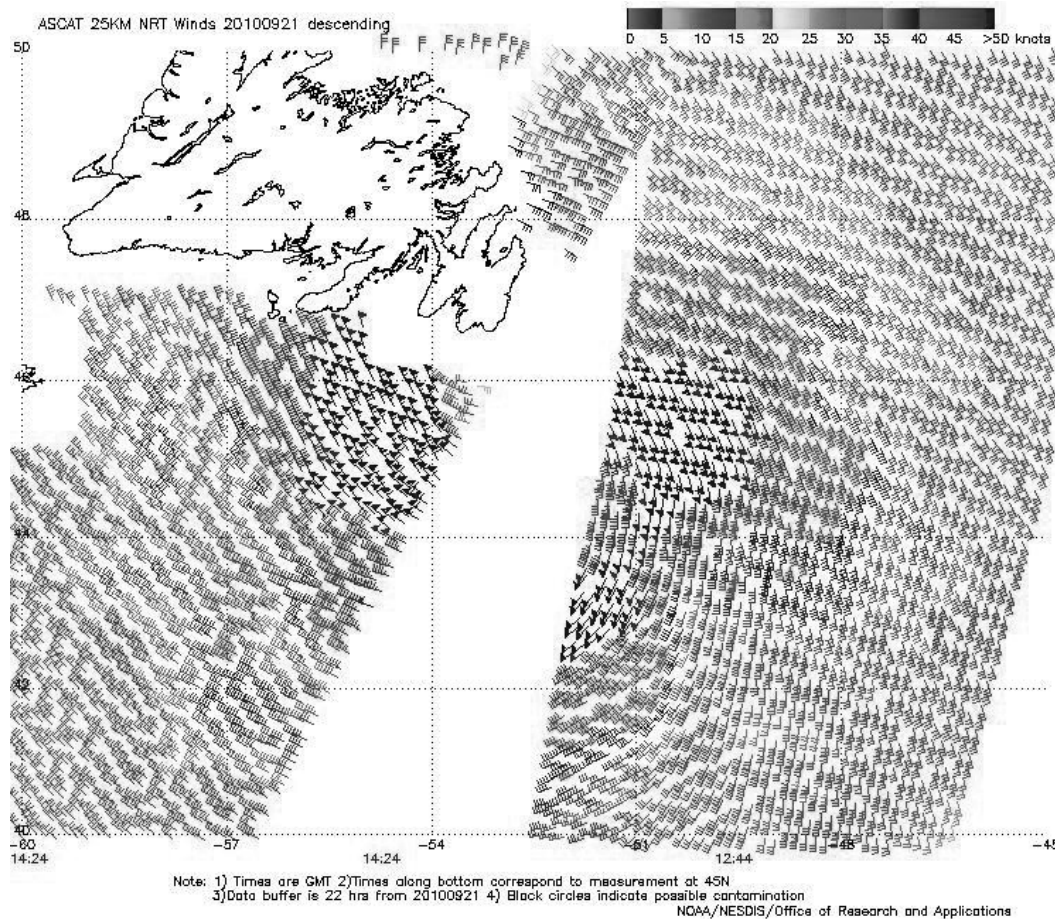
Figure 4. 25 km ASCAT (Advanced Scatterometer) image of satellite sensed winds around Hurricane Igor which was undergoing extratropical transition at this time. This is the higher resolution version of the imagery. Portions of two passes (1424 UTC and 1244 UTC September 21, 2010) are shown.
