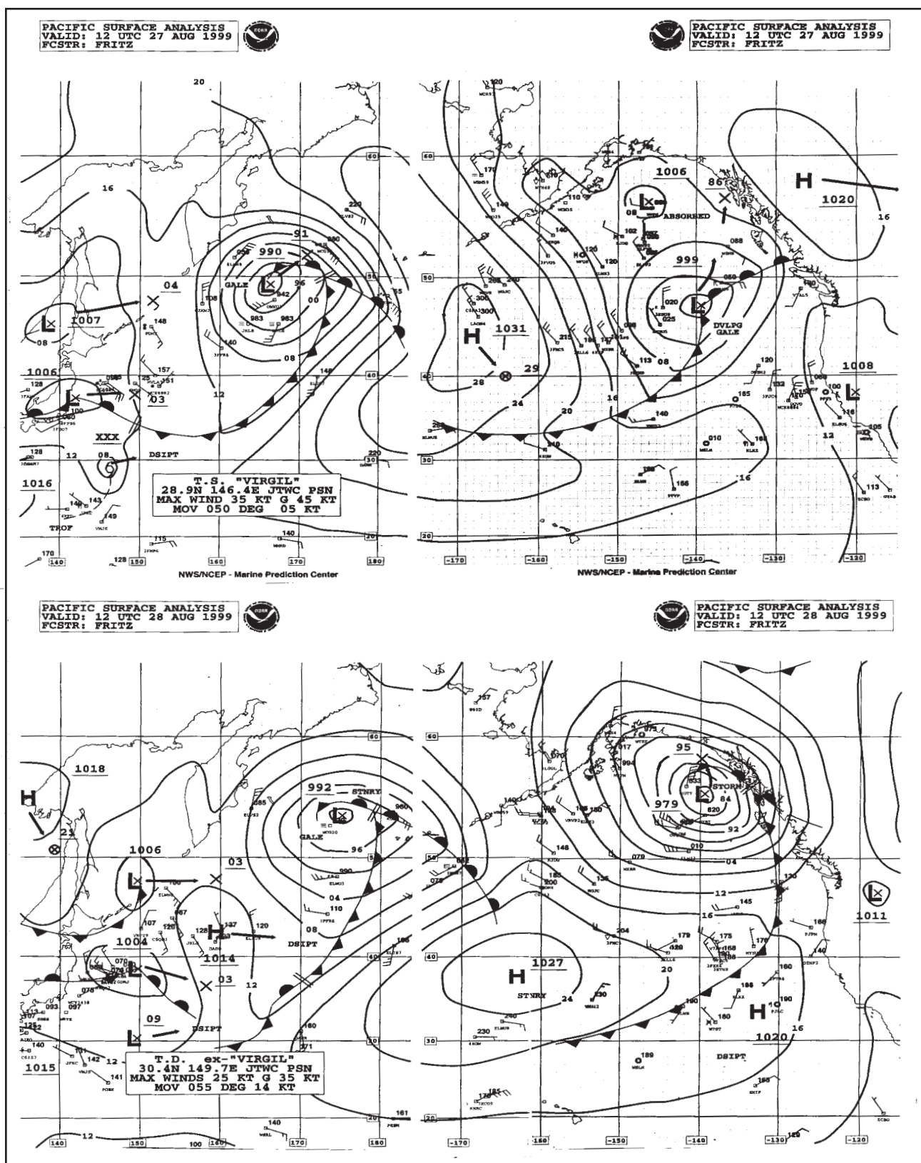
Figure 11. MPC North Pacific surface analyses valid 1200 UTC August 27 and 1200 UTC August 28, 1999.
