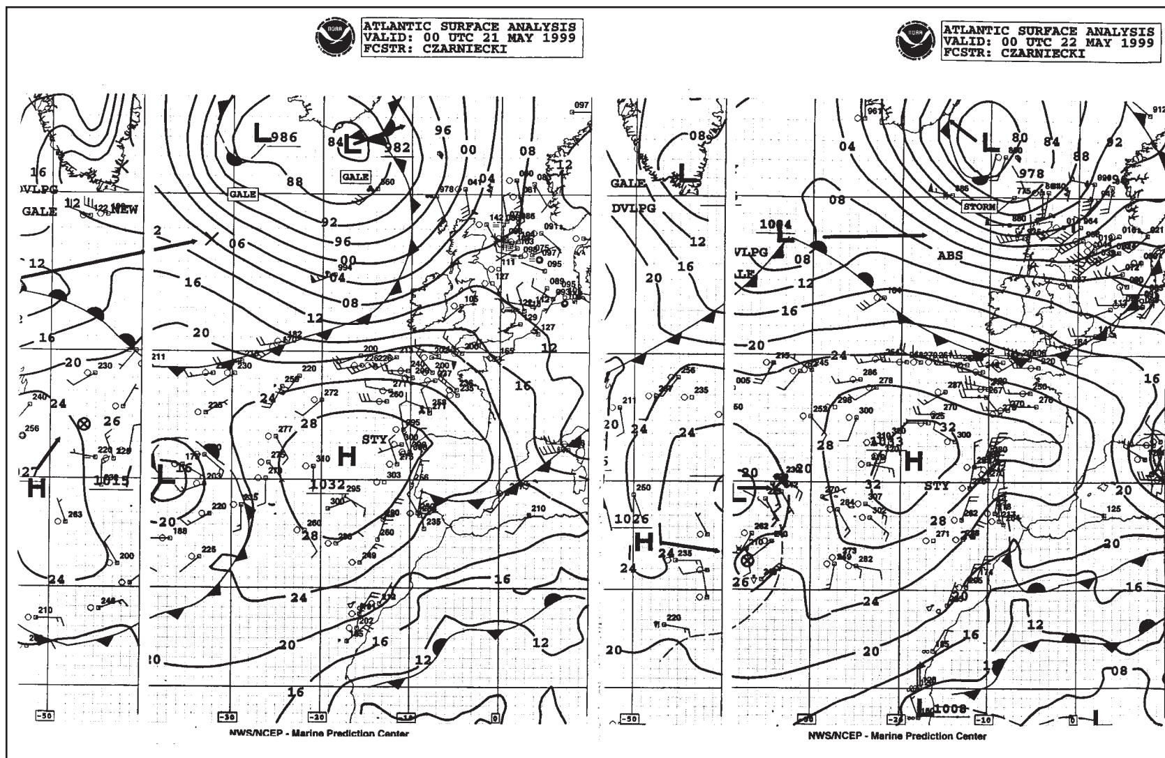
Figure 5. Series of two MPC Part I North Atlantic surface analyses valid at 0000 UTC on each of the dates May 21 and 22, 1999. Development of storm in far northeast Atlantic is shown.
