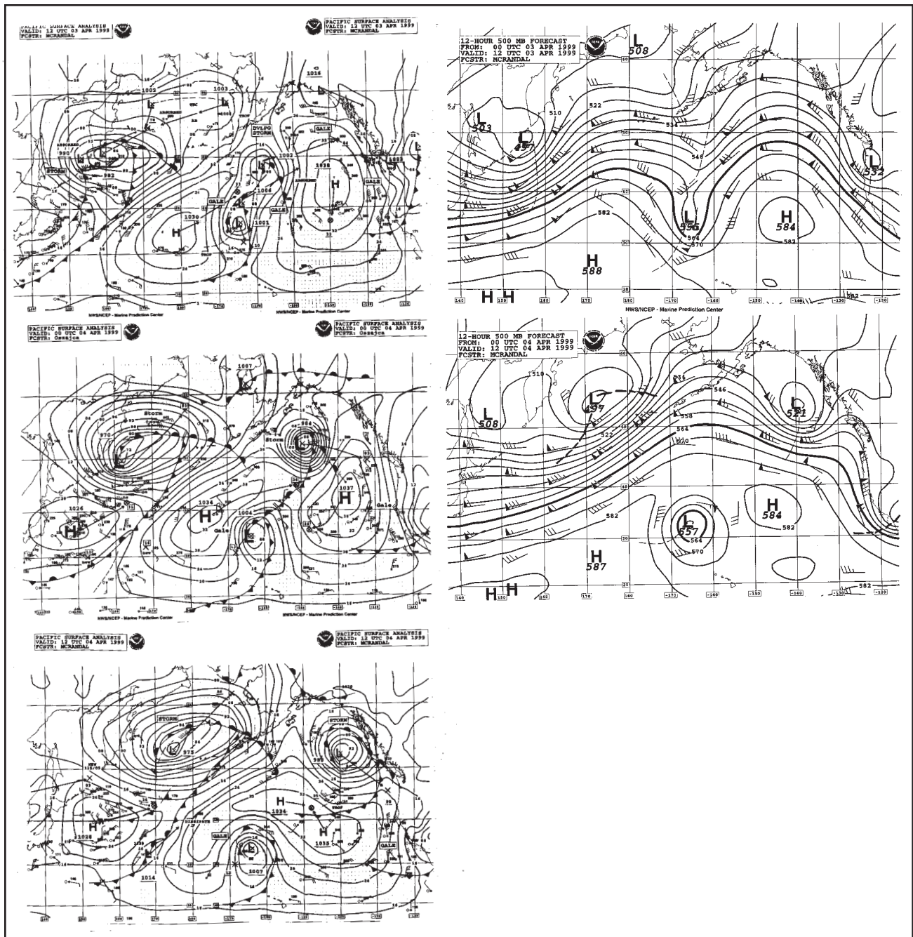
Figure 1. Series of three MPC Pacific surface analysis charts valid at 1200 UTC 03 April, 0000 UTC 04 April and 1200 UTC 04 April 1999. The 500-millibar charts (model-generated 12-hour forecasts with short wave troughs manually added) are valid 1200 UTC 03 April and 1200 UTC 04 April, matching the valid times of the first and third surface analyses.
