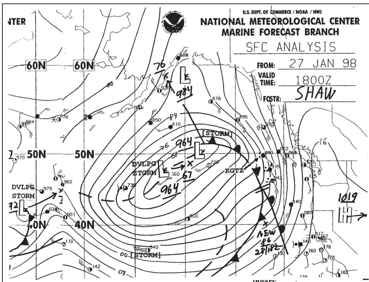
Figure 2. Surface analysis valid 18Z 27 January 1998 with arrow pointing to KGTZ observation.
