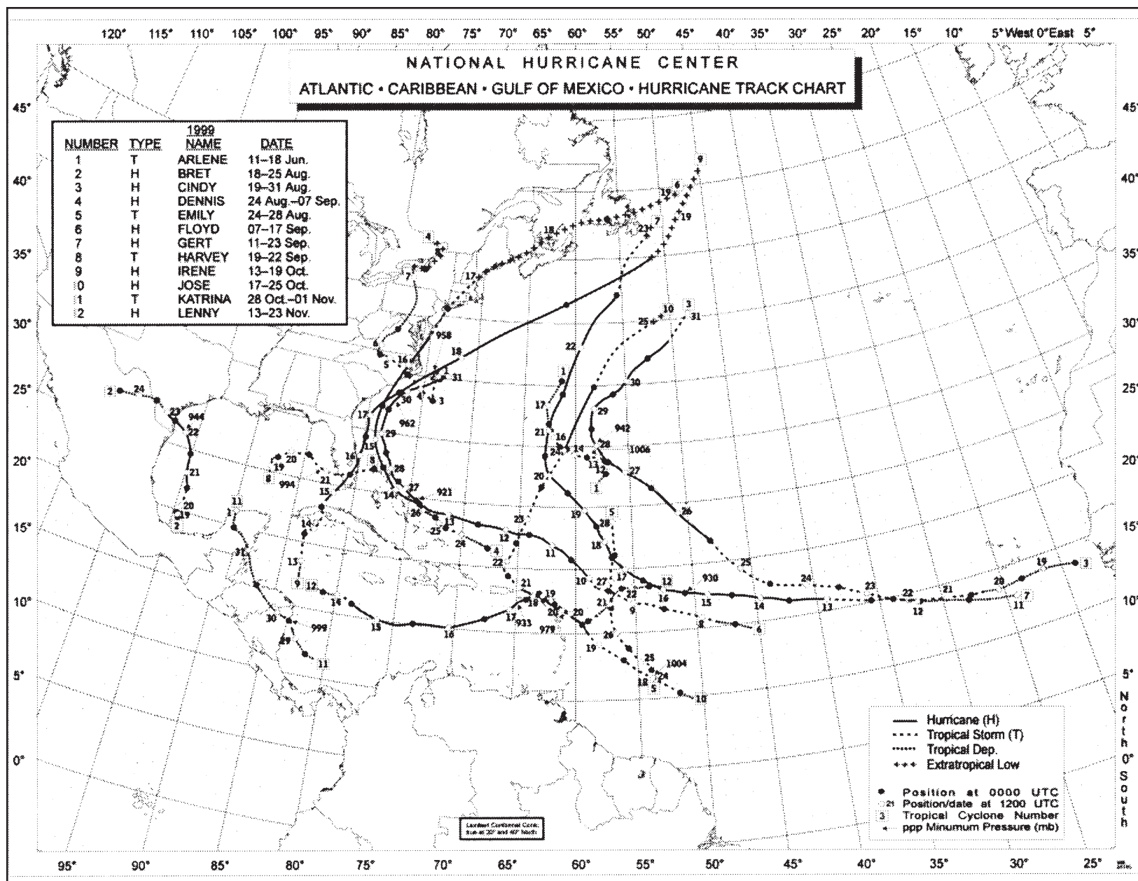
Figure 1. Atlantic hurricane and tropical storm tracks of 1999.
