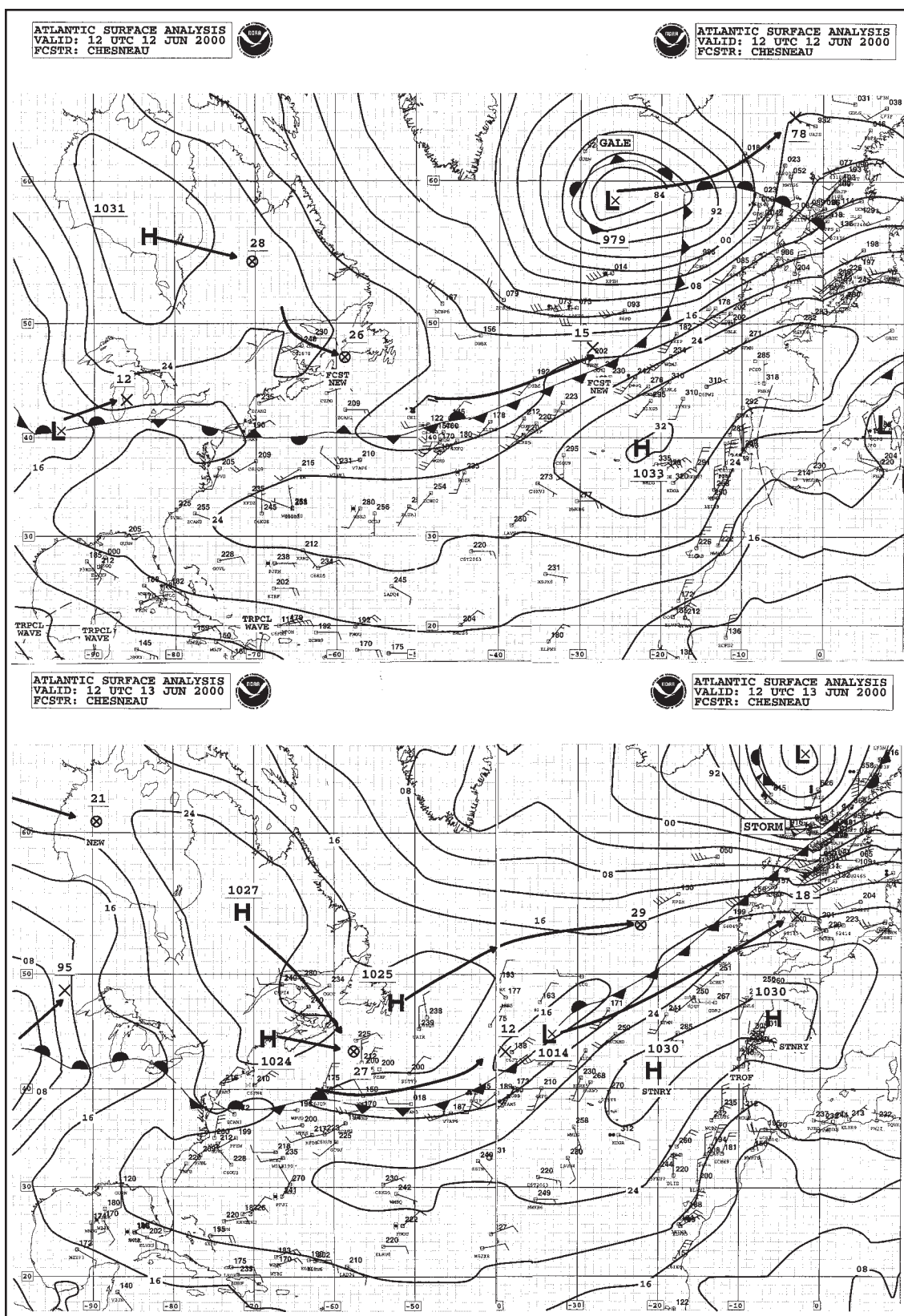
Figure 4. MPC North Atlantic surface analysis charts valid 1200 UTC 12 and 13 June 2000.
