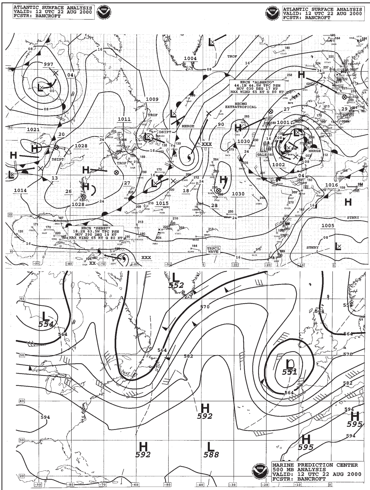
Figure 9. MPC North Atlantic surface analysis and corresponding 500-Mb analysis valid at 1200 UTC 22 August 2000.
