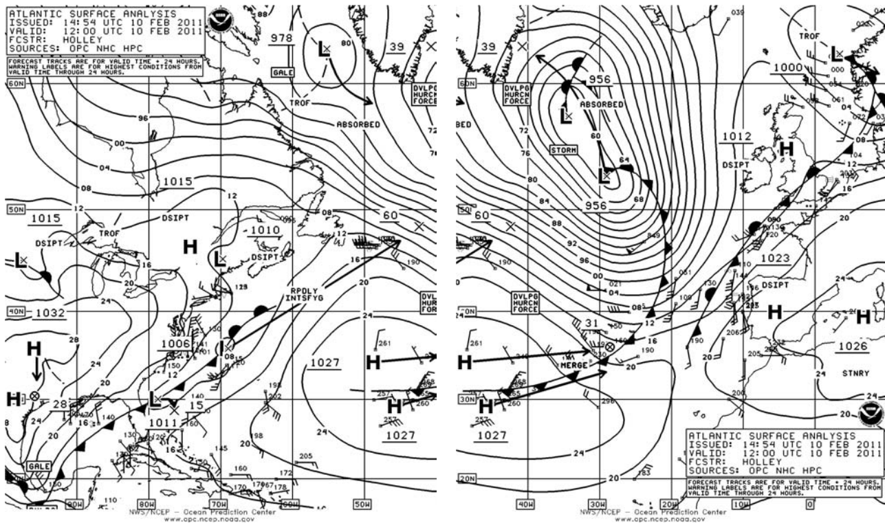
Figure 8. OPC North Atlantic Surface Analysis charts valid 1200 UTC February 10, 2011.
