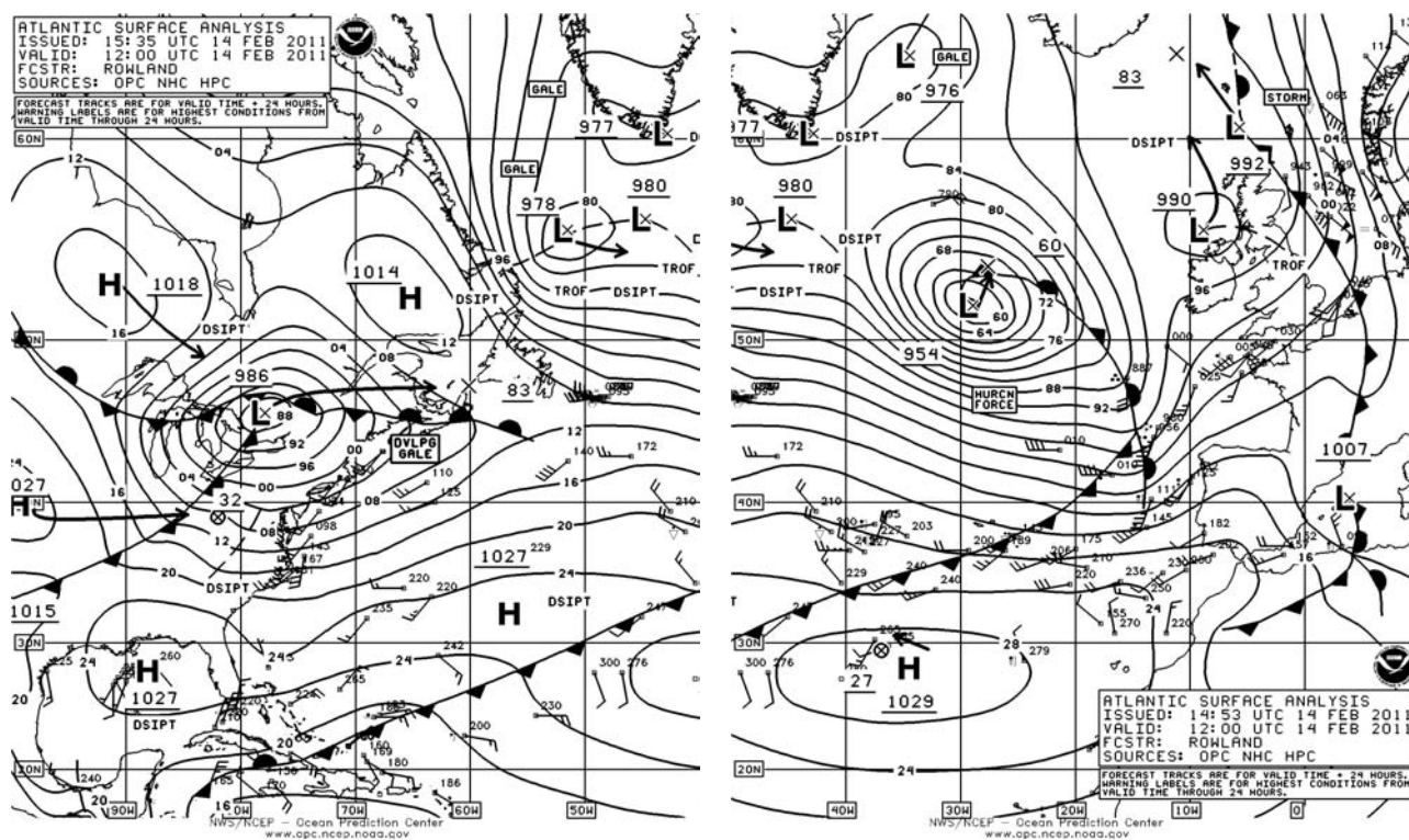
Figure 10. OPC North Atlantic Surface Analysis charts valid 1200 UTC February 14, 2011.
