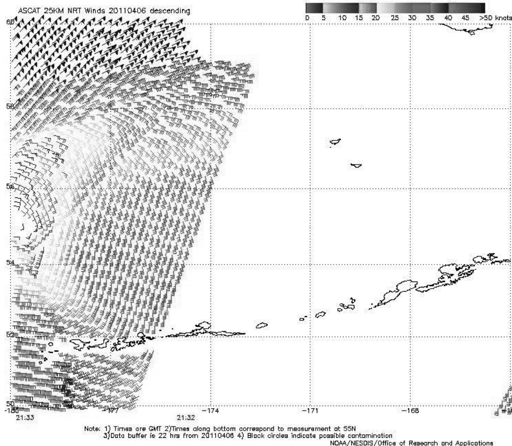
Figure 21. 25-km ASCAT image of satellite sensed winds around the east semicircle of the hurricane-force low shown in the second part of Figure 20. The valid time of the pass is 2133 UTC April 6th, 2011, or about two and one-half hours prior to the valid time of the second part of Figure 20. The center of the cyclone is near the western edge of the image. Image is courtesy of NOAA/NESDIS/ Center for Satellite Application and Research.
