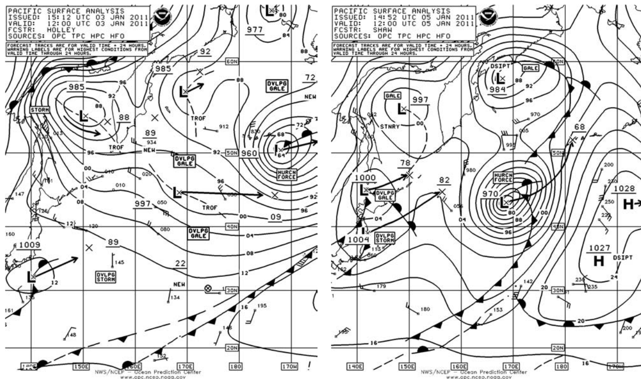
Figure 1. OPC North Pacific Surface Analysis charts valid 1200 UTC January 3rd and 5th, 2011. Twenty-four hour forecast tracks are shown with the forecast central pressures given as the last two whole digits in hPa, except XX for tropical cyclones.
