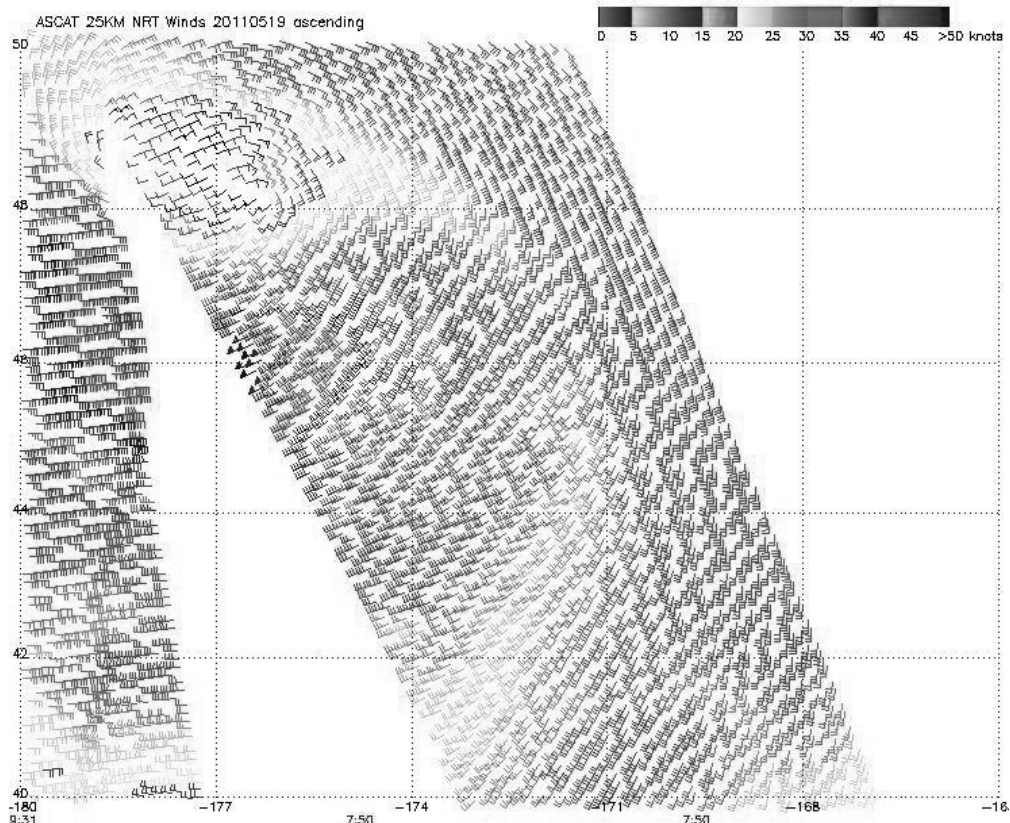
Figure 23. 25-km ASCAT image of satellite sensed winds around the storm shown in the second part of Figure 22. The valid times of the eastern pass is 0750 UTC and of the western pass 0931 UTC May 19th, 2011. The eastern pass is less than two hours later than the valid time of the second part of Figure 22. The center of the cyclone is in the upper left portion of the image.
