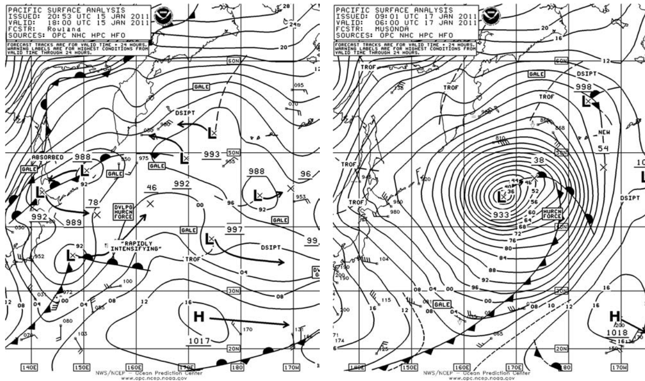
Figure 5. OPC North Pacific Surface Analysis charts valid 1800 UTC January 15th and 0600 UTC January 17th, 2011.
