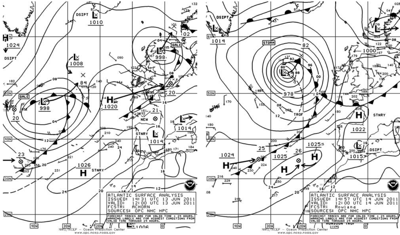
Figure 19. OPC North Atlantic Surface Analysis charts valid 1200 UTC June 13 and 14, 2011.
