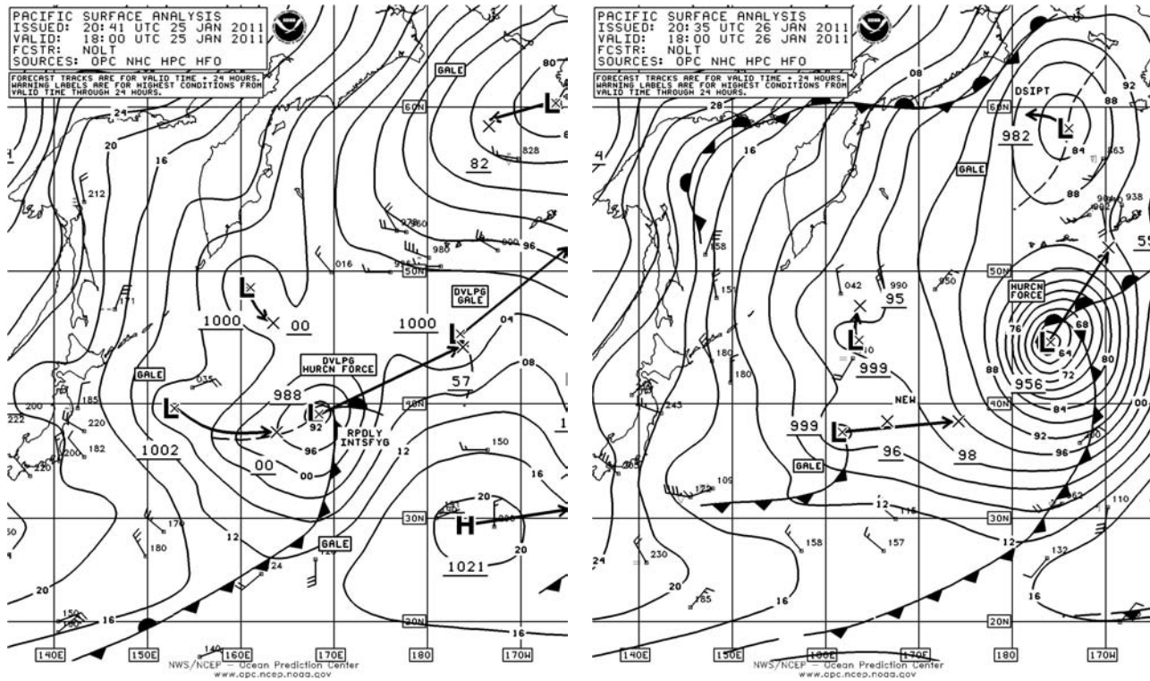
Figure 8. OPC North Pacific Surface Analysis charts valid 1800 UTC January 25th and 26th, 2011.
