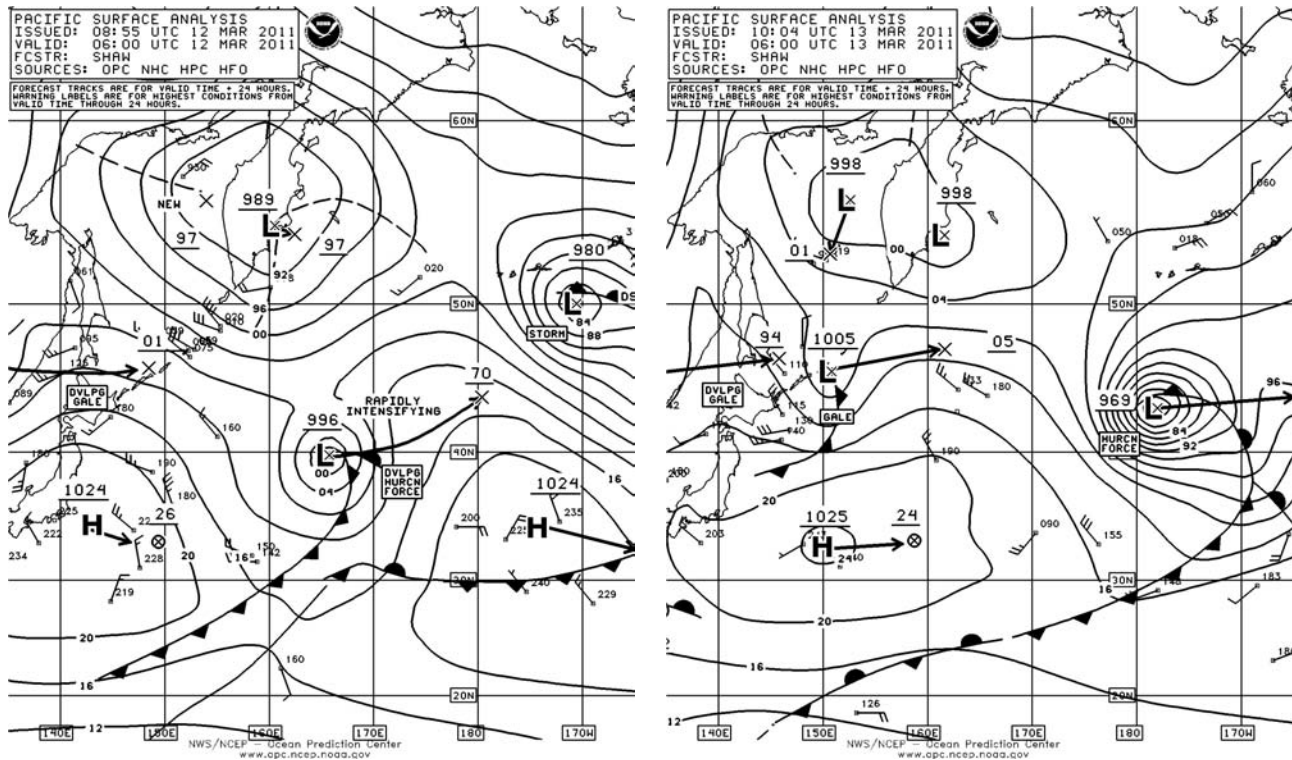
Figure 14. OPC North Pacific Surface Analysis charts valid 0600 UTC March 12th and 13th, 2011.
