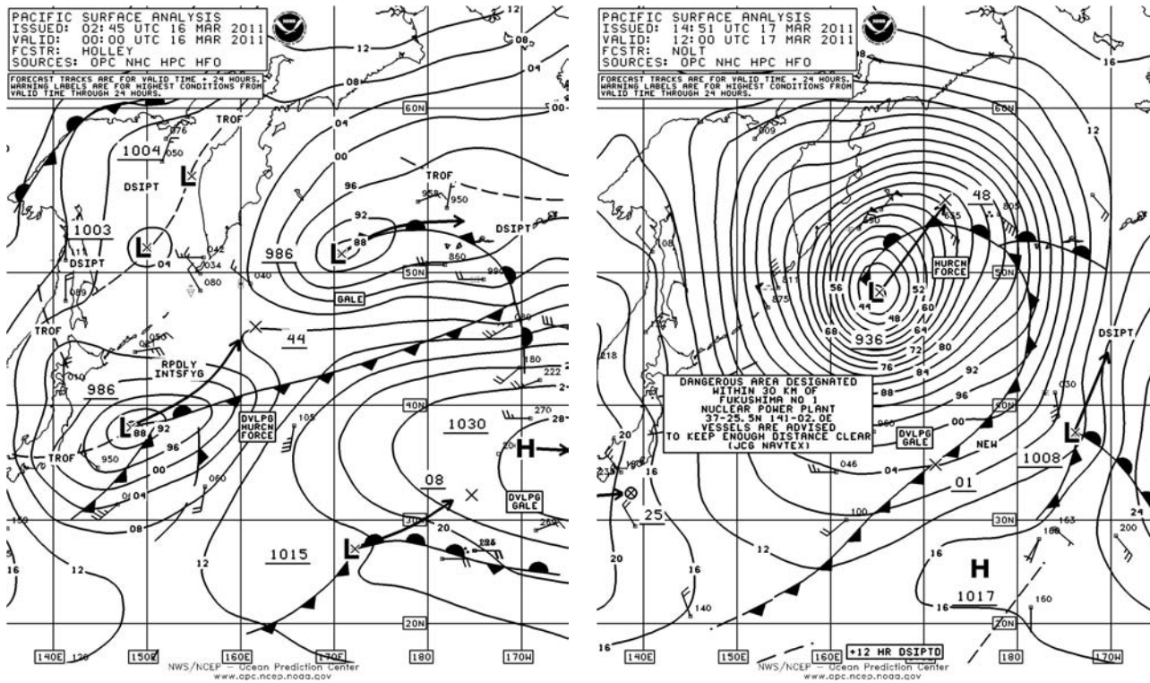
Figure 16. OPC North Pacific Surface Analysis charts valid 0000 UTC March 16th and 1200 UTC March 17th, 2011.
