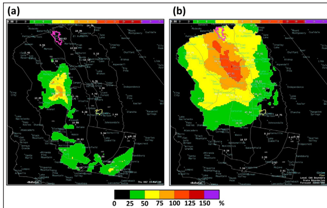
Figure 3. Select images generated from the EPFT in Fig. 2 displaying the spatial extent of the QPF/ARI 100 values from the a) 6-hr HIRSWRFnm valid starting at 0000 UTC 22 March 2018 (max=95%) and b) 24-hr CMCnh valid starting 0000 UTC 22 March 2018 (max=126%). The magenta outline depicts the bounds of the Detwiler burn scar.
