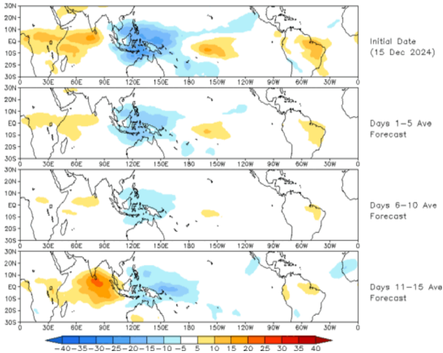
Prediction of MJO-related anomalies using GEFS operational forecast Initial date: 15 Dec 2024 OLR
