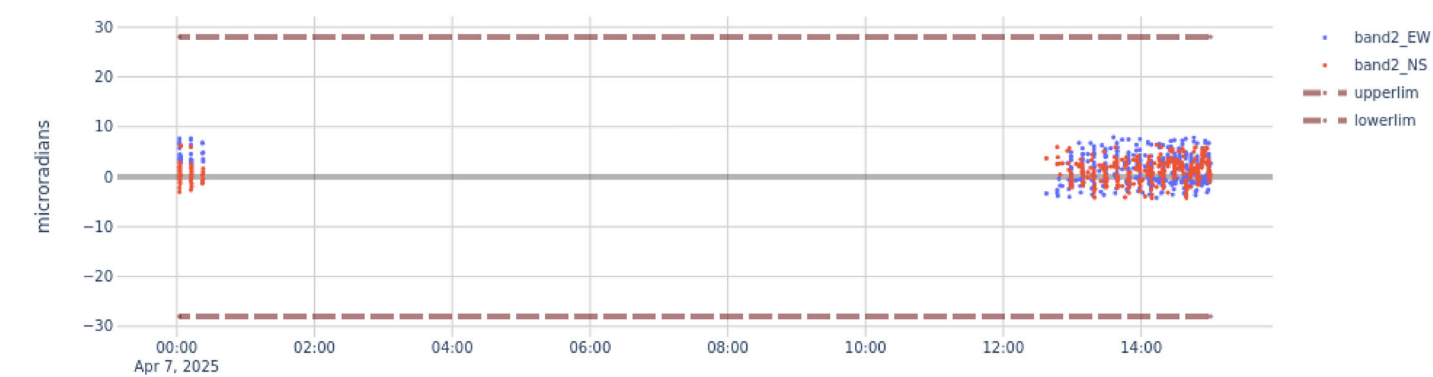
NAV Residuals plot Band:2 [INR.merged]
