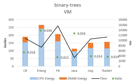
Figure 1. Energy and time graphical data for binary-trees
