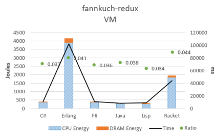
Figure 2. Energy and time graphical data for fannkuch-redux
