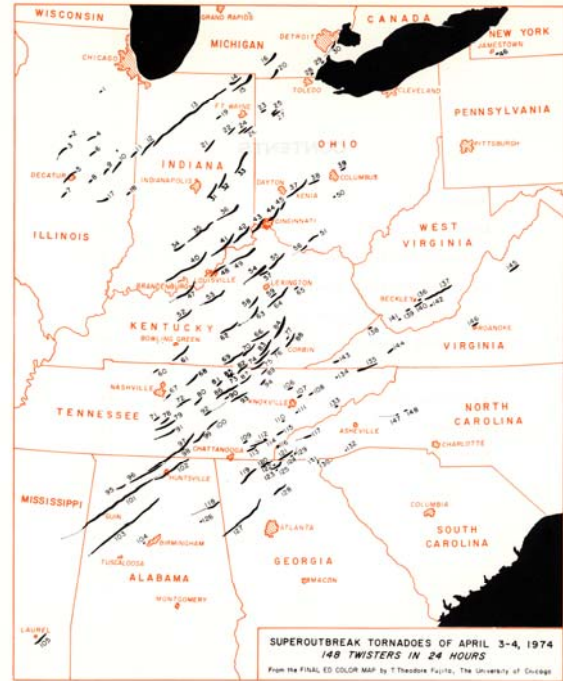
Figure 1. Tracks of the 148 Super Outbreak tornadoes documented by Fujita (1975).
