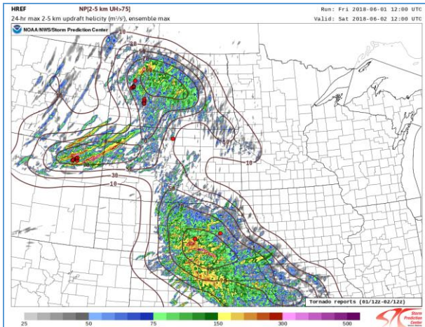
Figure 15. Same as Fig. 13, except for 12 UTC 1 June 2018.
