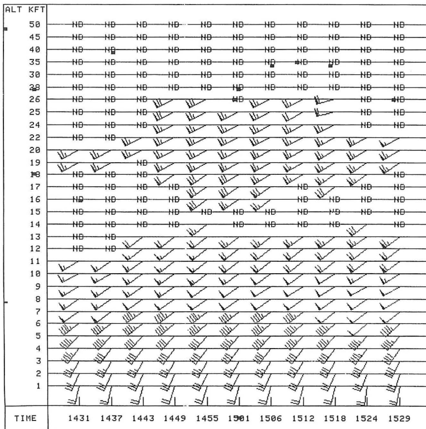
Fig. 22. Time series (UTC) of the VAD Wind Profile (VWP) product from the Maxwell Air Force Base, Alabama WSR-88D (KMXF). Wind barbs and flags are the same as in Fig. 11.
