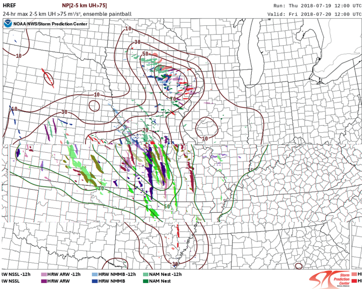
FIG. 3. From the 1200 UTC 19 Jul 2018 cycle of the HREFv2, the paintball plot for 2–5 km UH >75 \text{m}^2 \text{ s}^{-2} over the 24-h period from 1200 UTC 19 Jul to 1200 UTC 20 Jul 2018. Contours of NMEP for 2–5 km UH >75 \text{m}^2 \text{ s}^{-2} (the same field plotted as color fill in Fig. 2) are overlaid.
