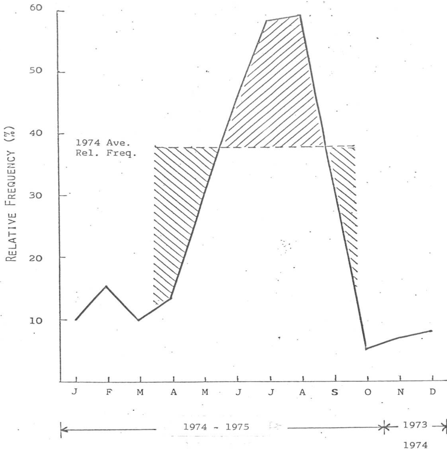
Figure 2. Relative frequency of MDR code \geq 4 for one MDR block in Southern Alabama for 0000 GMT \pm 3 hrs.
