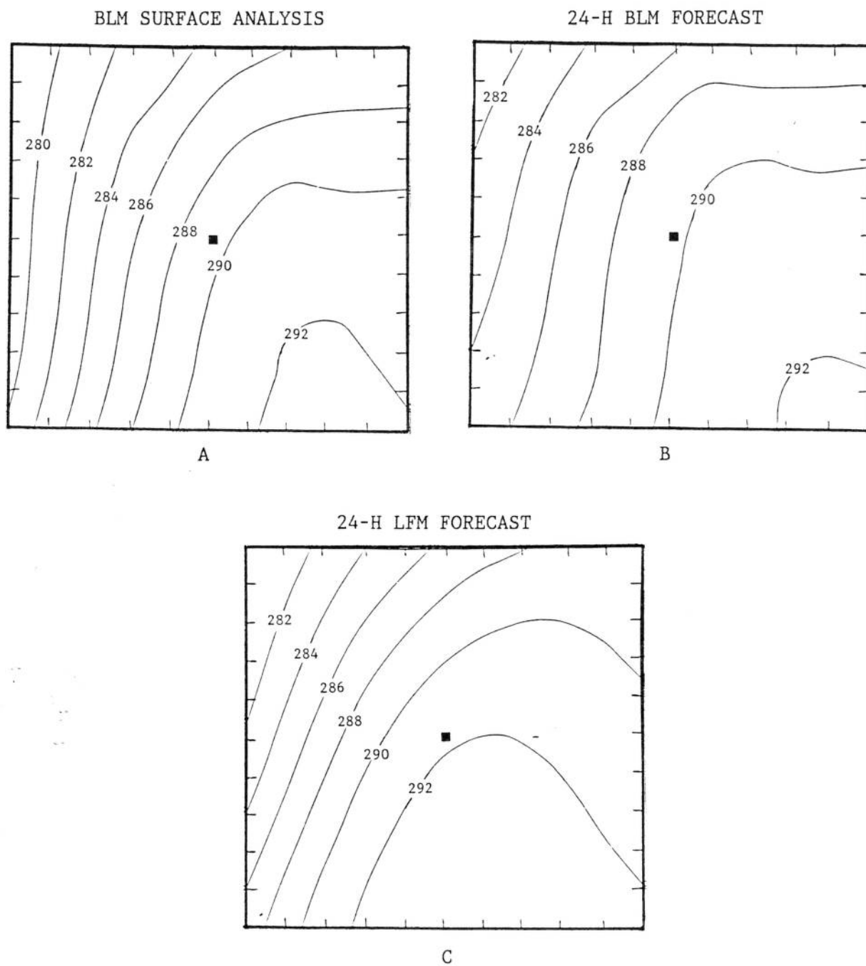
Figure 2. Composite surface dewpoint, K, from BLM analyses, BLM 24-h forecasts, and LFM 24-h forecasts. Tick marks represent distances of 80 km in this and similar figures.
