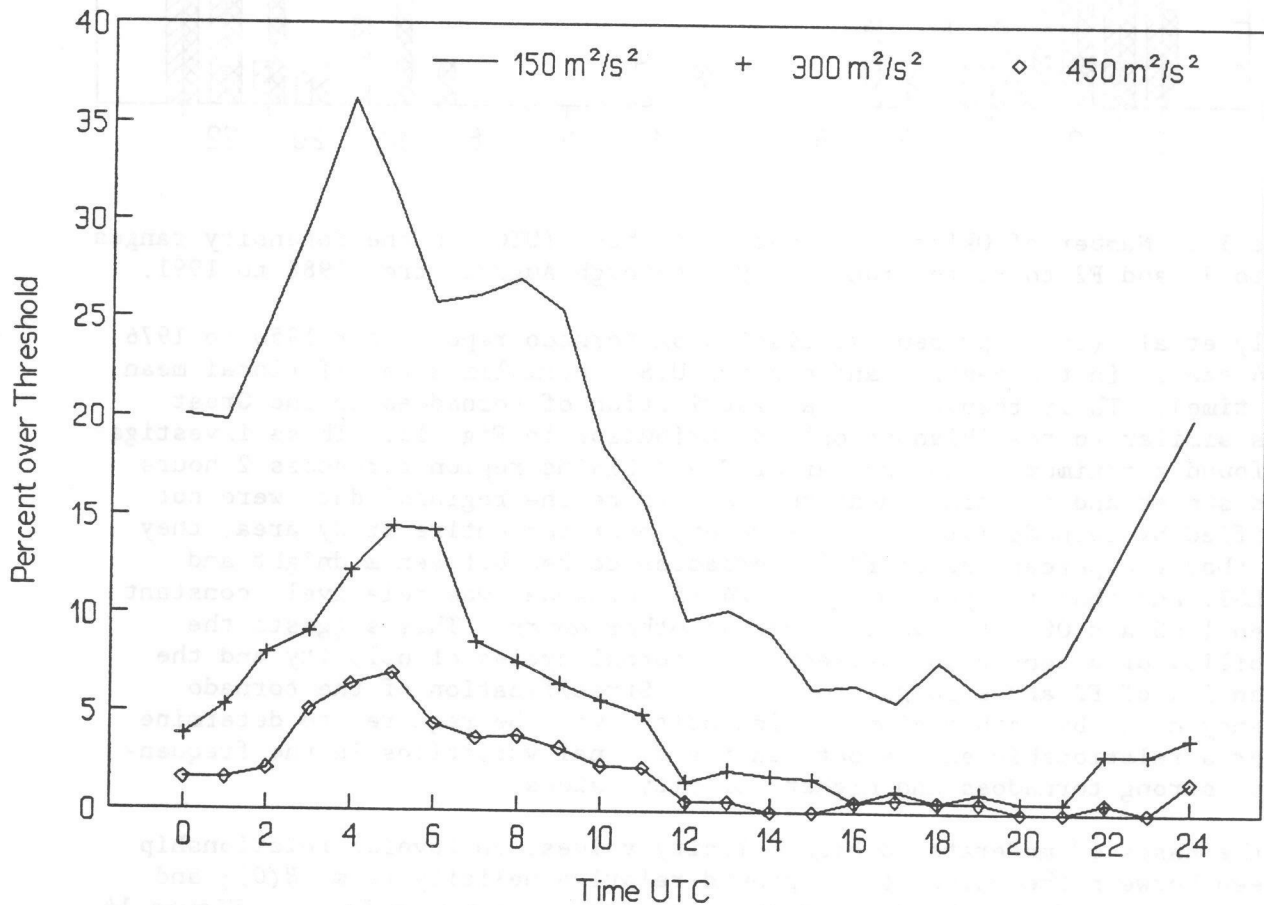
Figure 12. Percent of hourly storm-relative helicities that exceed each of three critical thresholds ( 150 , 300 , and 450 \text{ m}^2/\text{s}^2 ). Helicity is computed for the same data and in the same manner as in Fig. 11.
