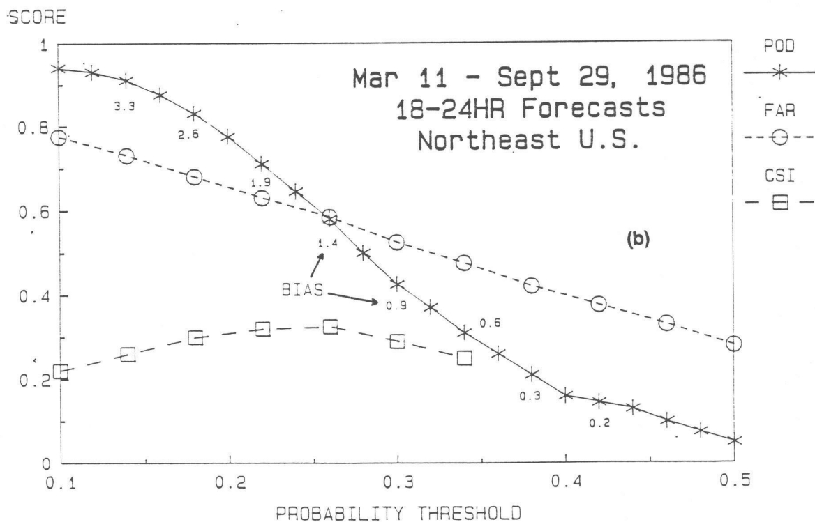
Figure 2. (a) Observed frequency of two or more lightning strikes per 47 km grid blocks as a function of forecast probability for 1987; (b) critical success index (CSI), false alarm ratio (FAR), and probability of detection (POD) for categorical thunderstorm occurrence based on various probability thresholds.
