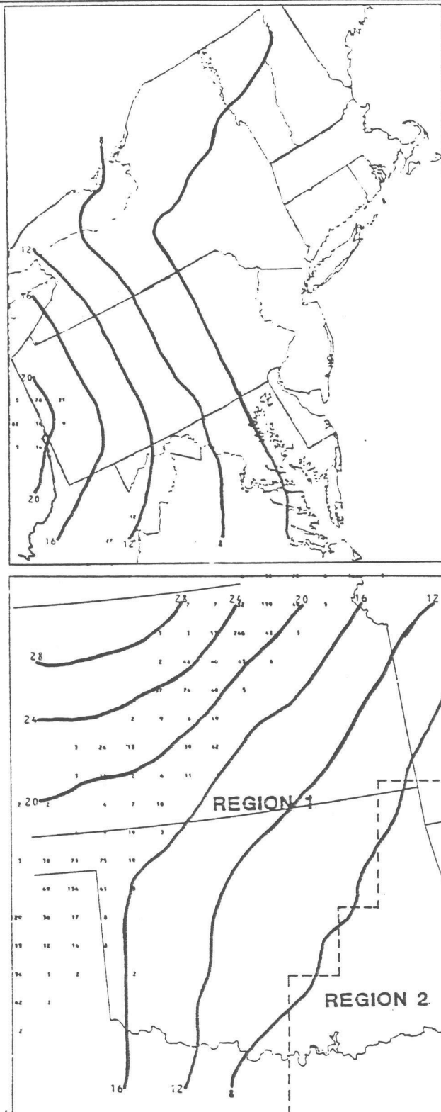
Figure 1. Probability of two or more lightning ground strikes during 18-24 h projection following 0000 UTC on June 4, 1986 for northeast U.S. (top) and 6-12 hr projection following 0000 UTC on May 26, 1987 for Kansas-Oklahoma region (bottom). Number of reported ground strikes is plotted for each 47 km grid block with two or more strikes. Region 1 and Region 2 designate geographical areas for which separate forecast equations were developed.
