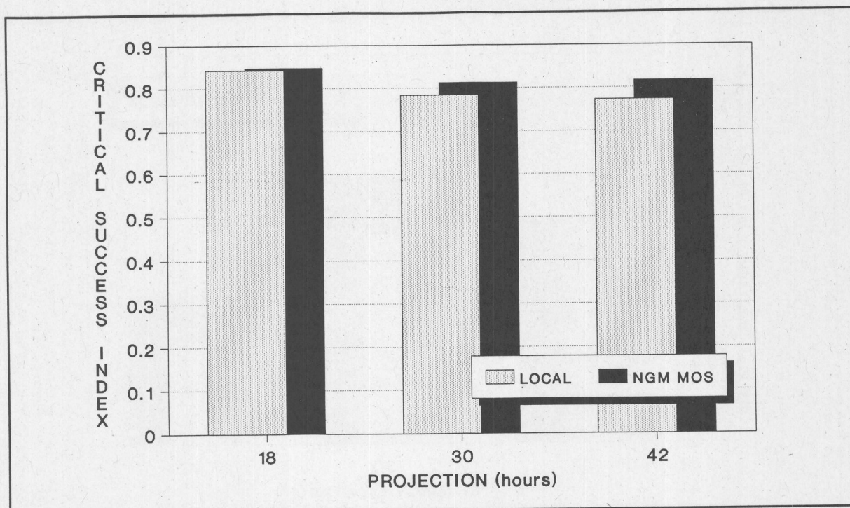
Figure 9. Critical success index for the local and NGM MOS snow category forecasts based on 0000 UTC data, October 1, 1993 to March 31, 1994.
