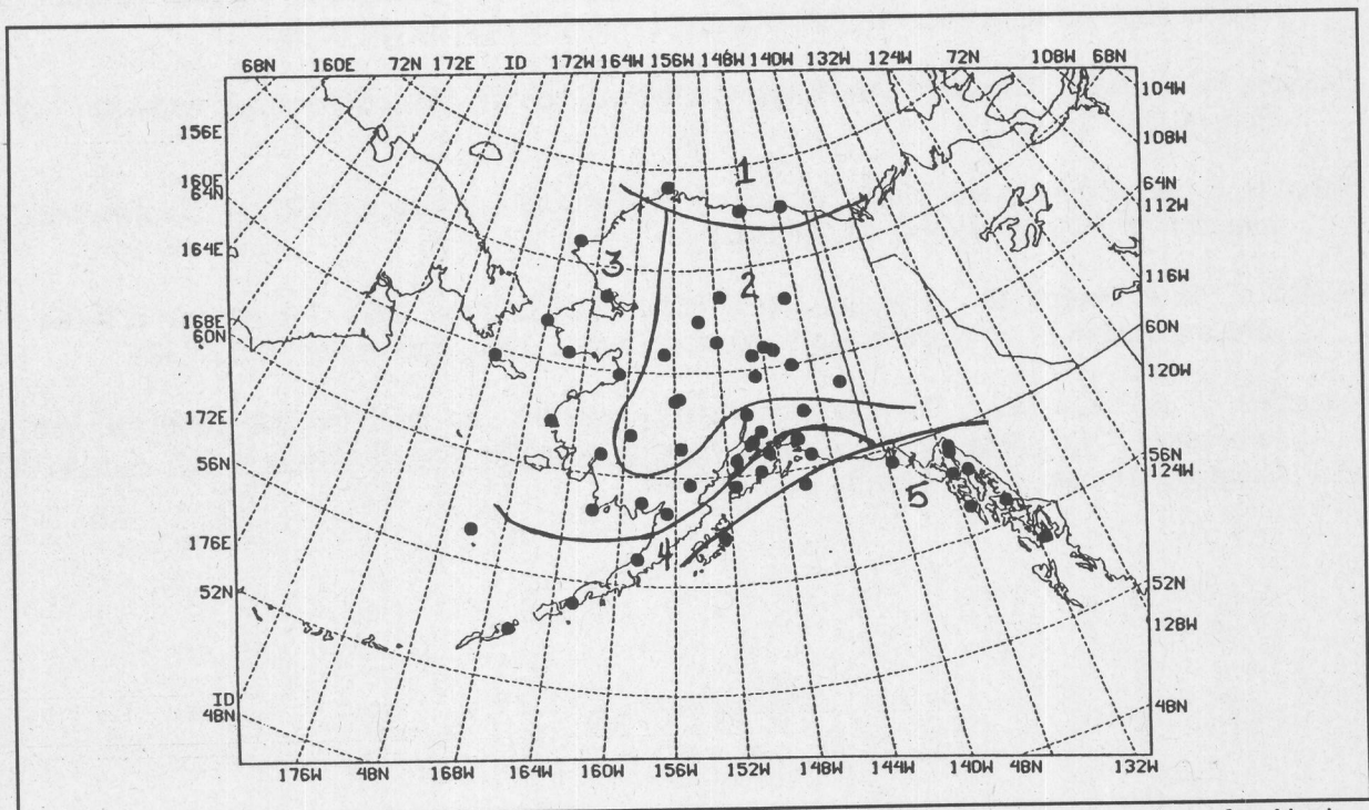
Figure 2. Regions used in the development of NGM precipitation type forecast equations for Alaska.
