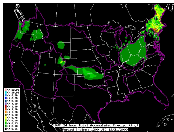
Figure 2a. NPVU 24-h QPE mosaic for hydrologic day ending at 1200 UTC 31 December 2000.
