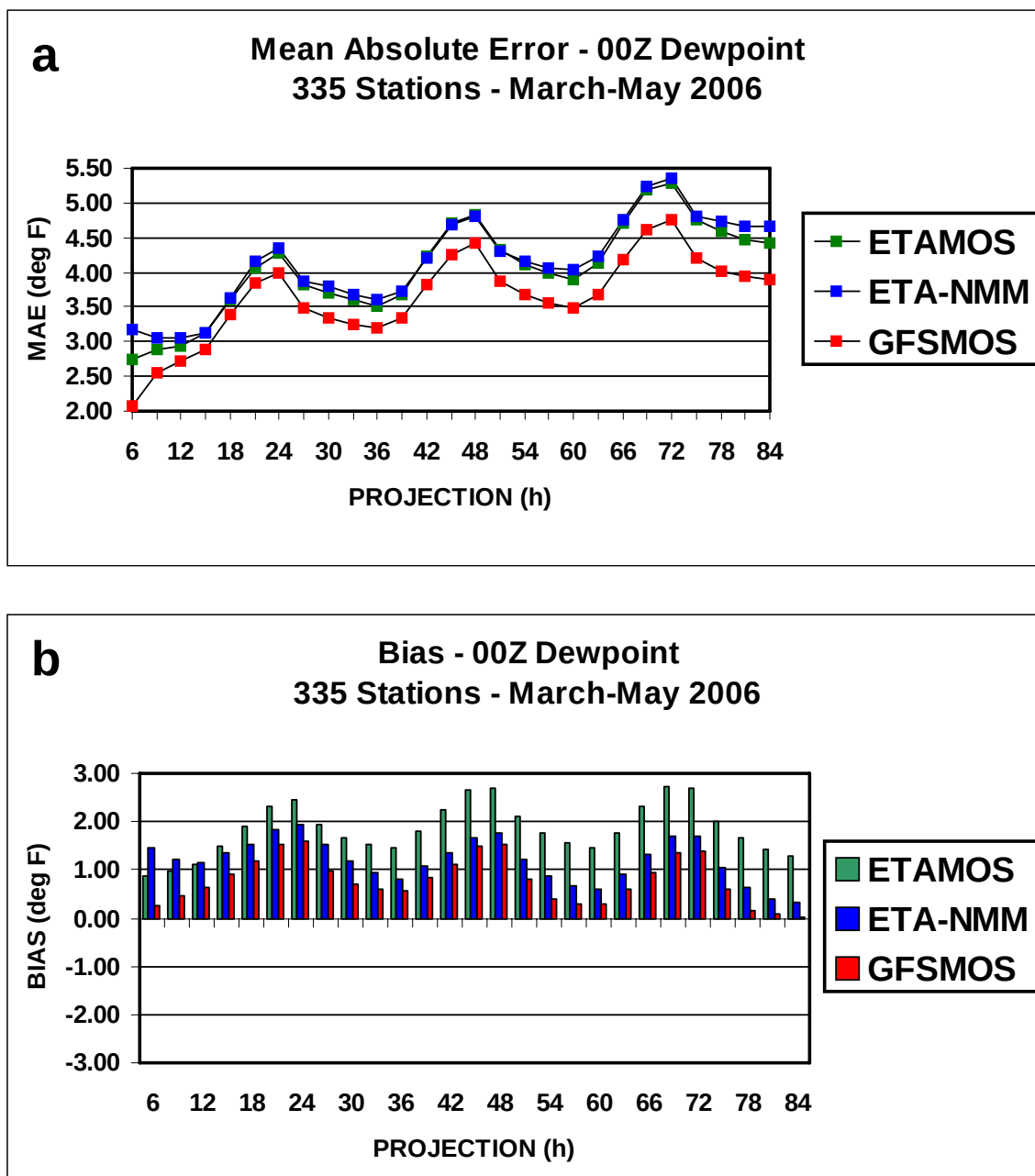
Figure 3. As in Fig. 1, but for (a) 2-m dewpoint MAE ( ^{\circ}\text{F} ) and (b) 2-m dewpoint bias ( ^{\circ}\text{F} ).
