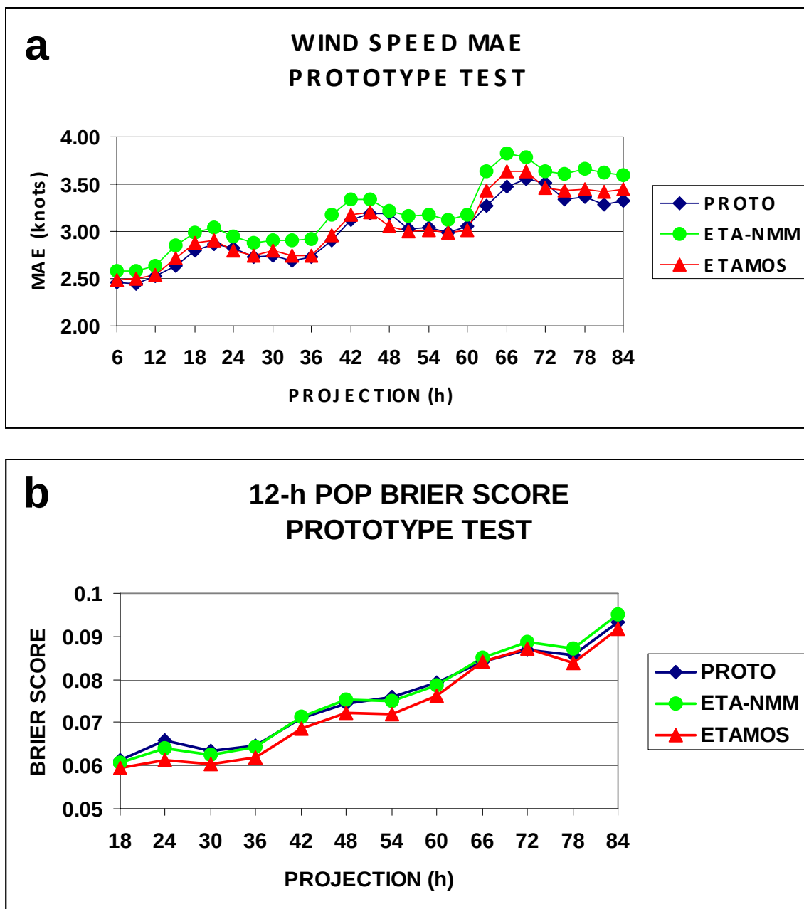
Figure 8. NAM MOS prototype results for (a) 10-m wind speed MAE (knots) and (b) 12-h PoP Brier score.
