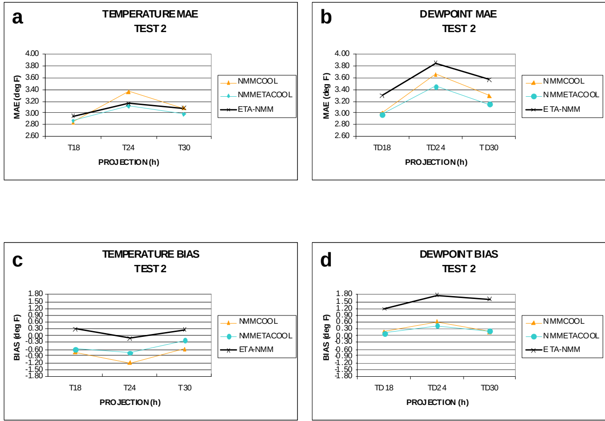
Figure 6. Same as in Fig. 5, but for Test 2.
